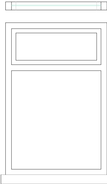
EXISTING SIDE ELEVATION TOP HUNG CASEMENT WINDOW
