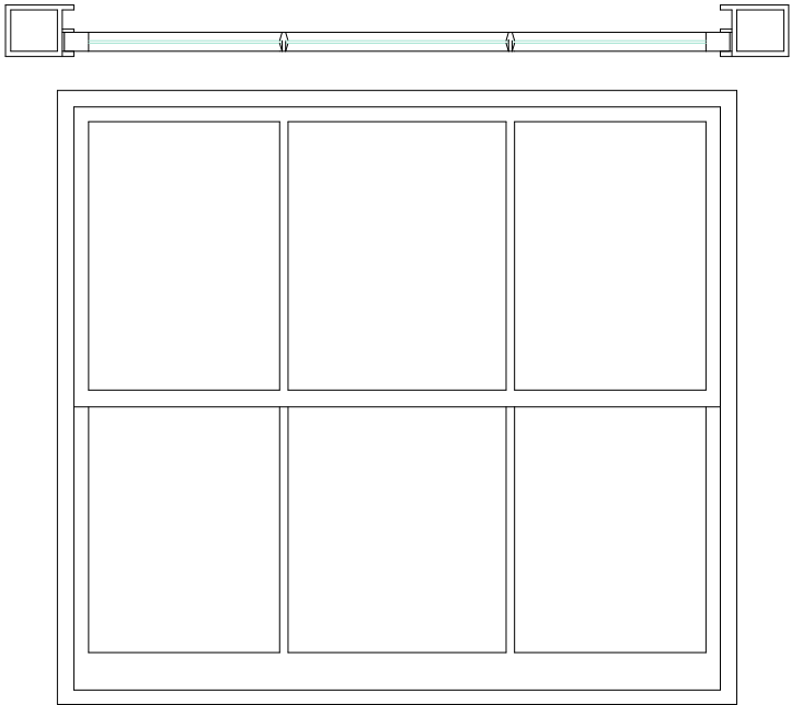
EXISTING FRONT BAY WINDOW
