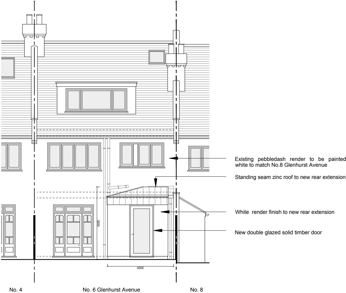
REAR ELEVATION
