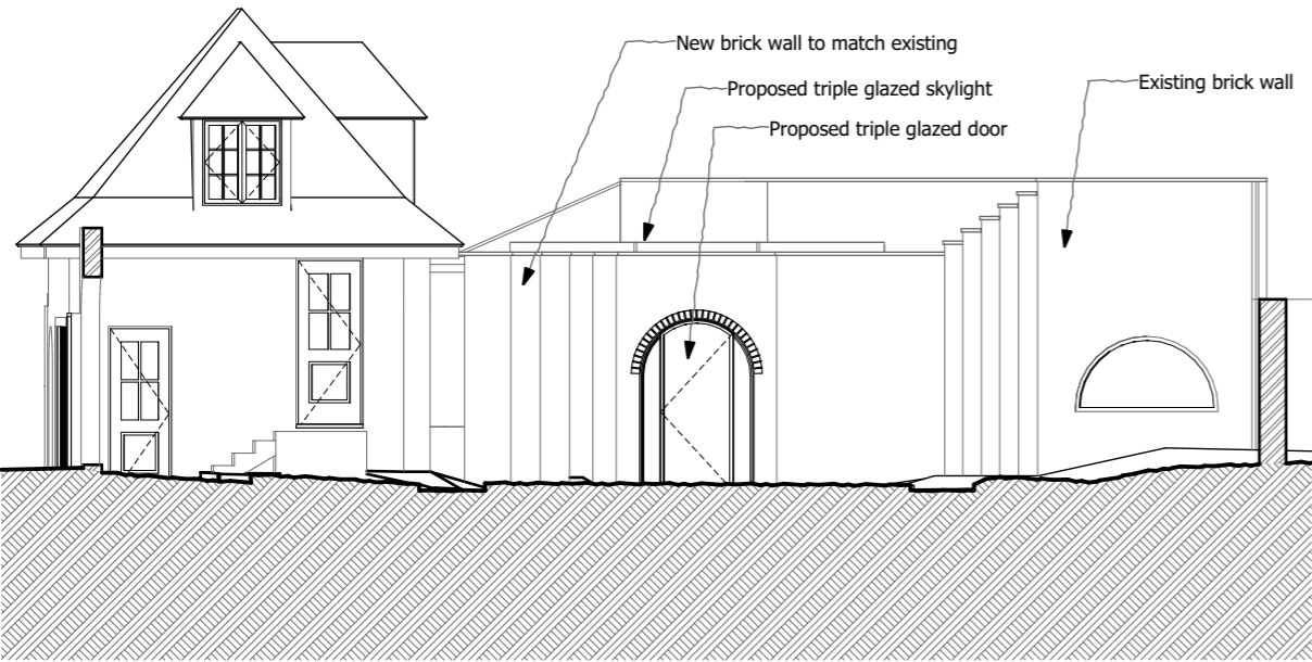
3 North Elevation Proposed 1:100
