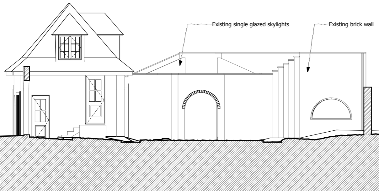
1 North Elevation Existing 1:100
