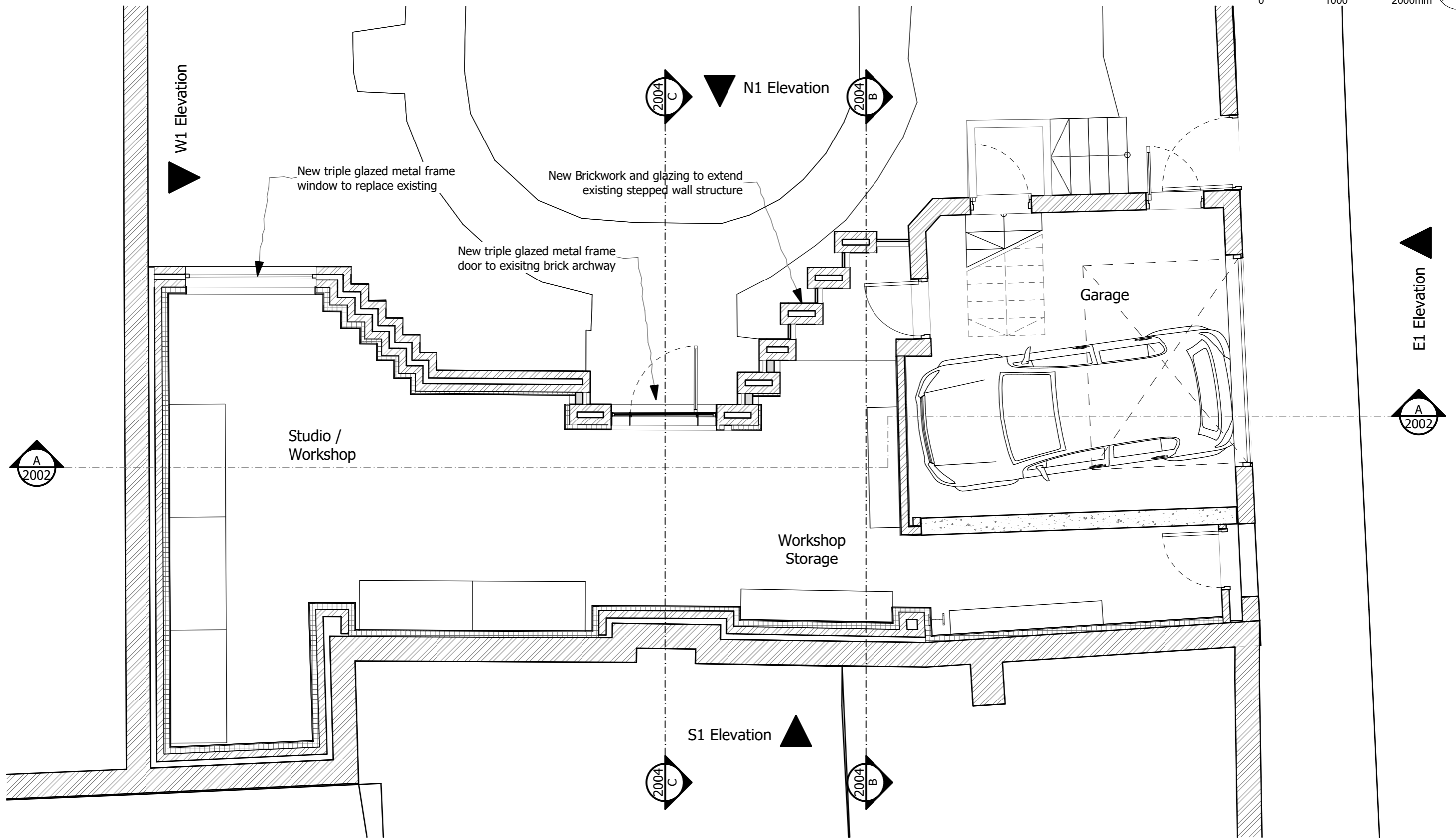
1 Ground Floor Proposed 1:50
