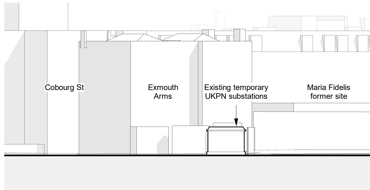
1 Elevation - North - Existing UKPN Substations 022311 1 : 200
