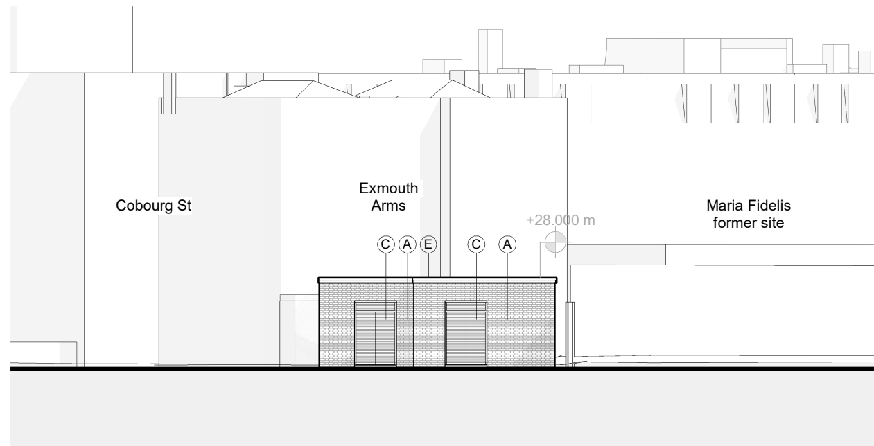
1 Elevation - North - Proposed UKPN Substation 000219 1 : 200
