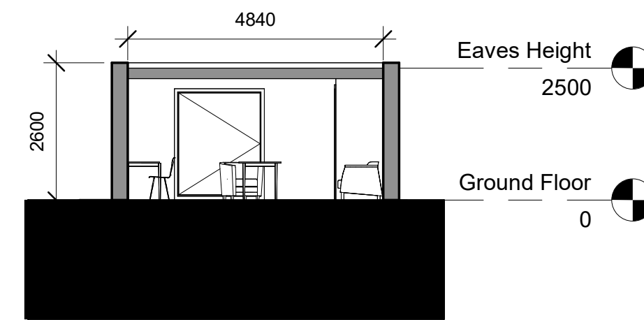
Proposed Cross Section 2-2
