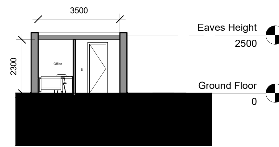
Proposed Cross Section 3-3
