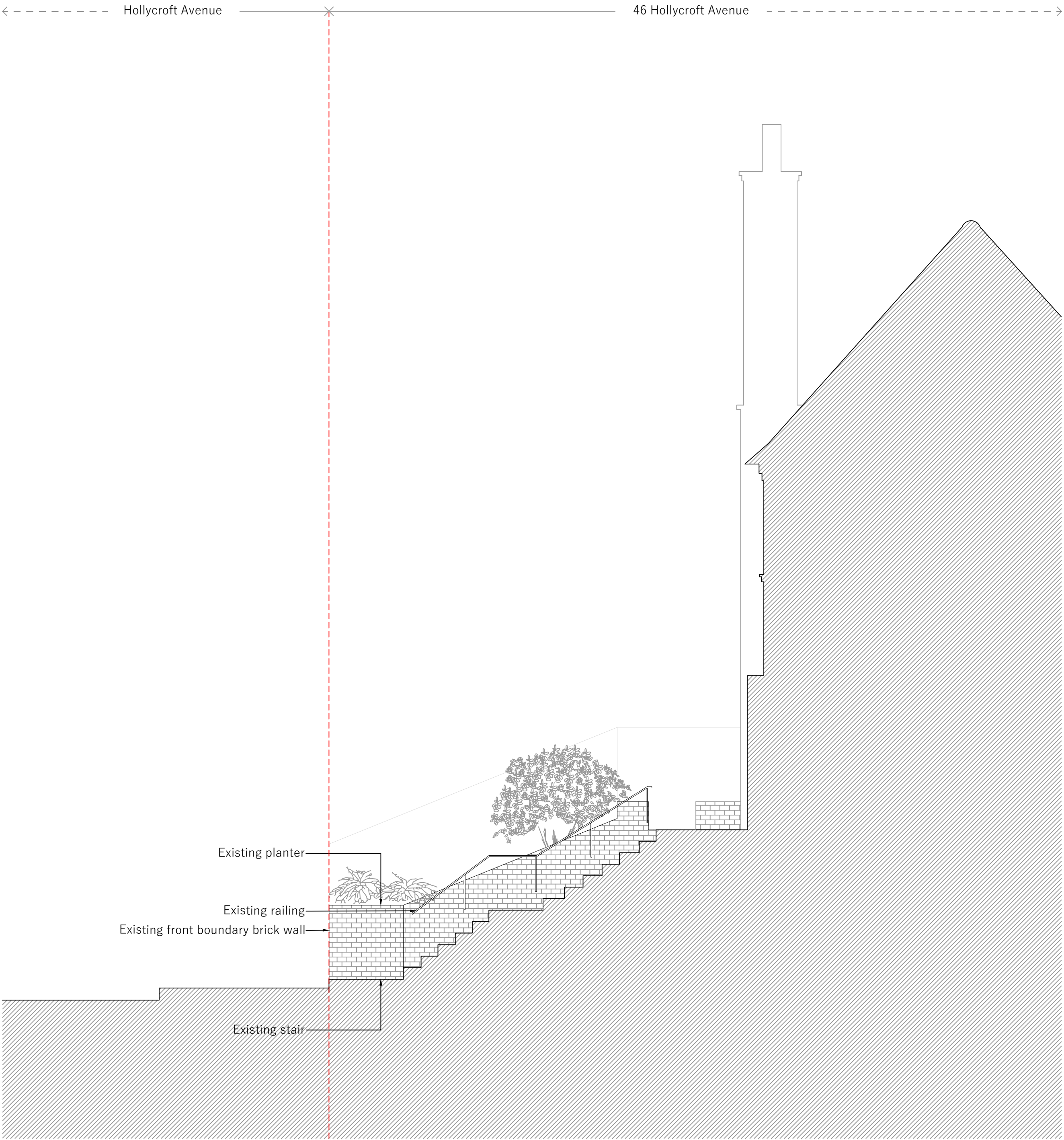
2 Existing short section 2
