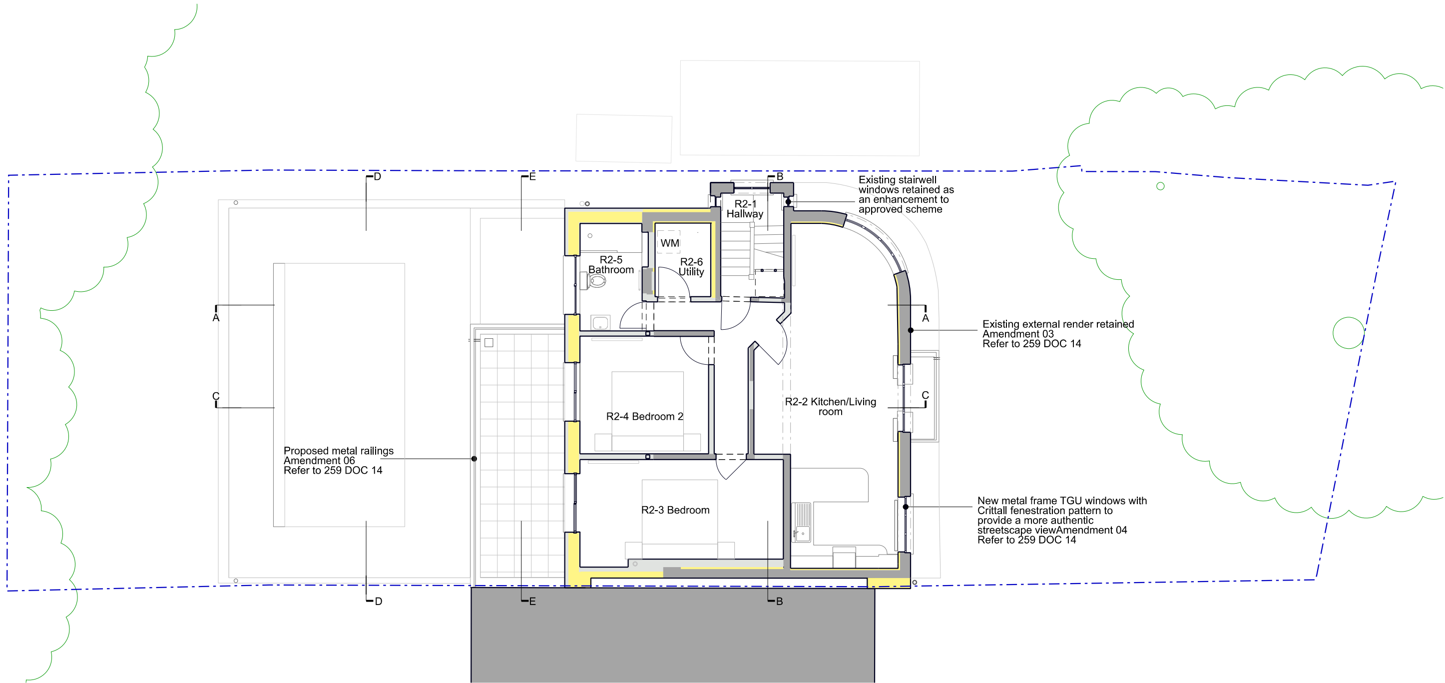
As Proposed Second Floor Plan
