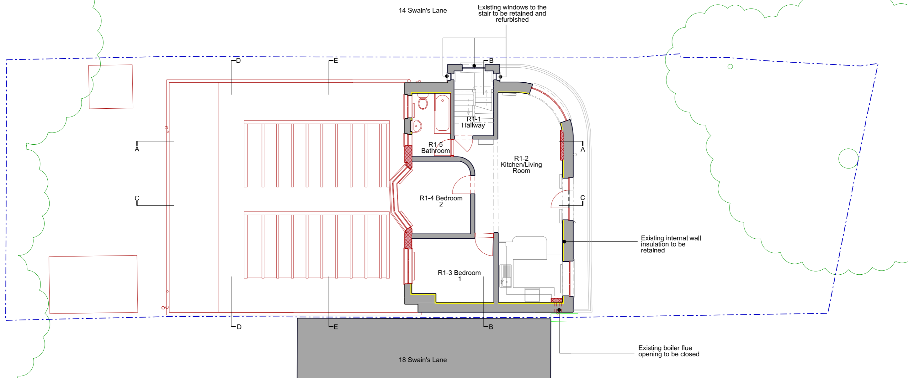
As Existing First Floor Plan
