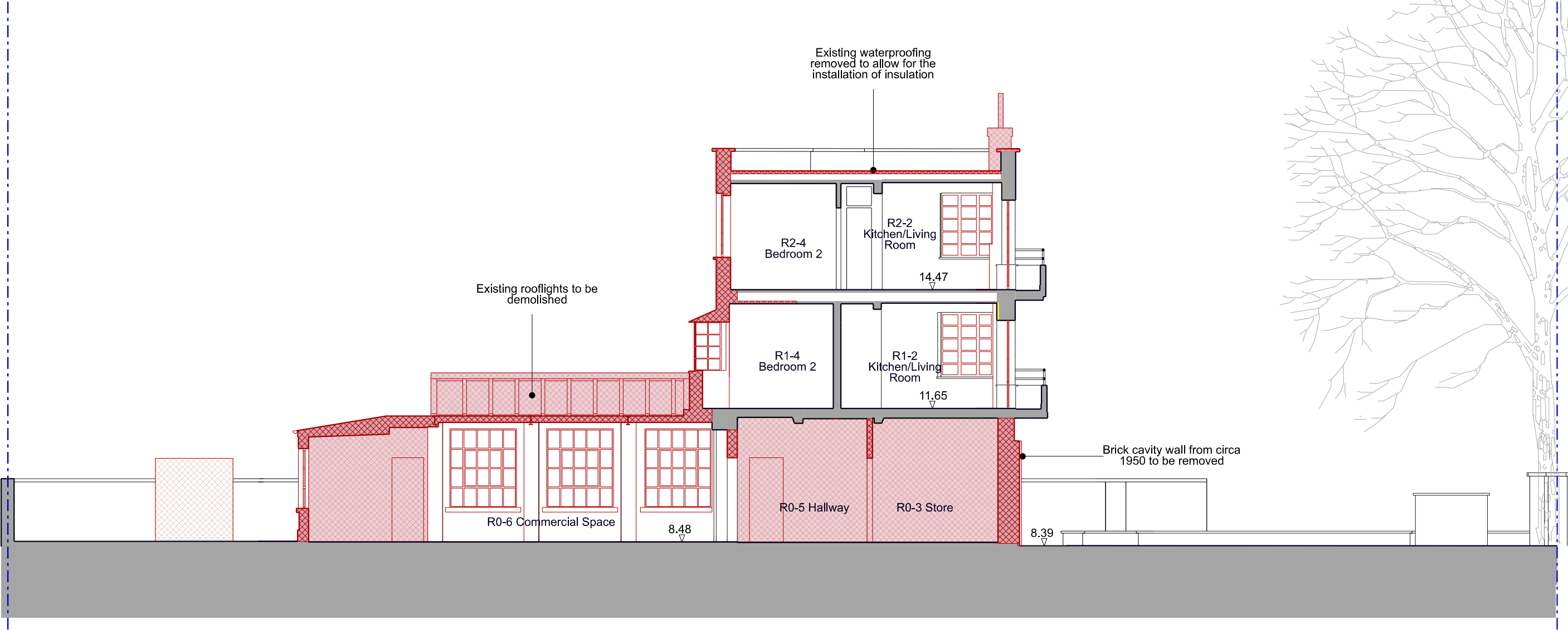
As Existing Section CC
