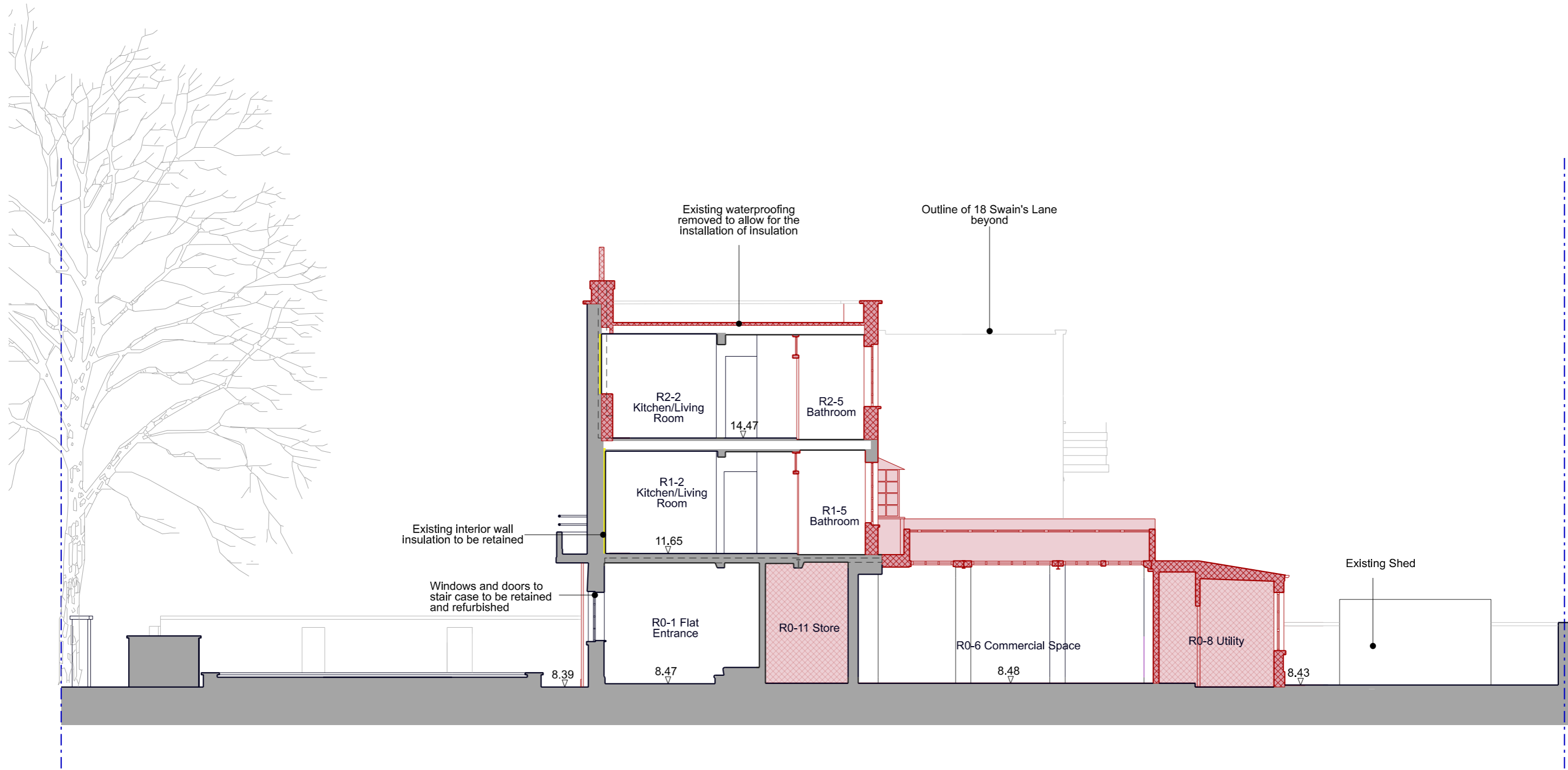
As Existing Section AA
