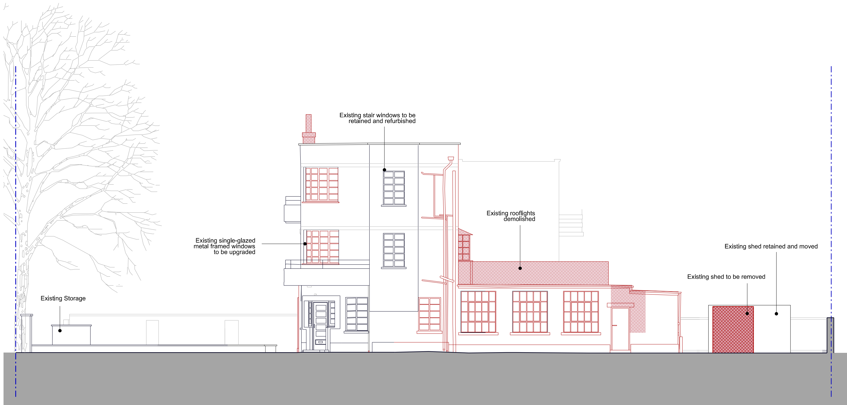
As Existing West Elevation
