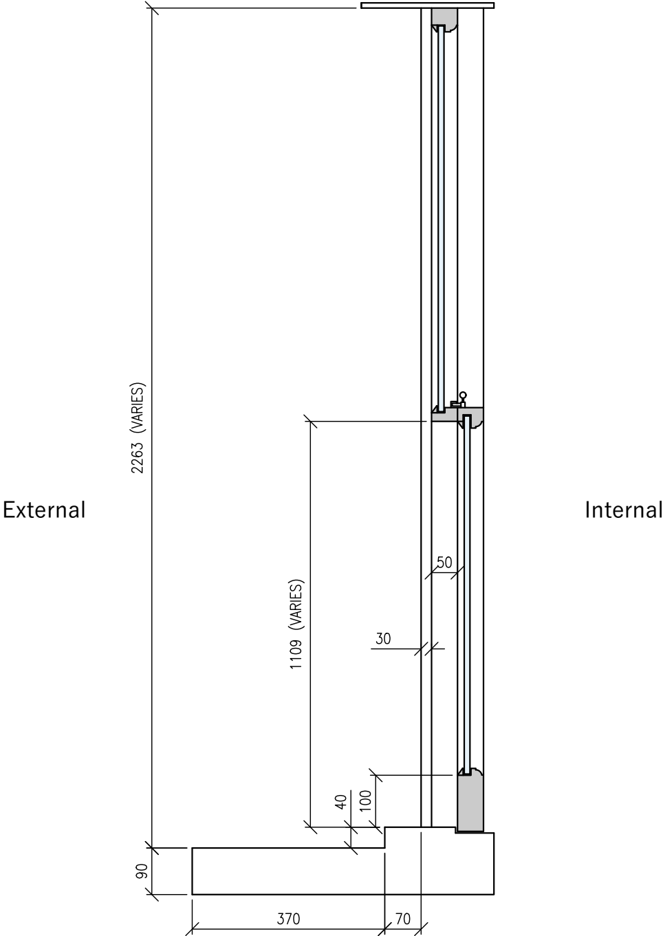
Typical Cross Section of Existing Sash Window
