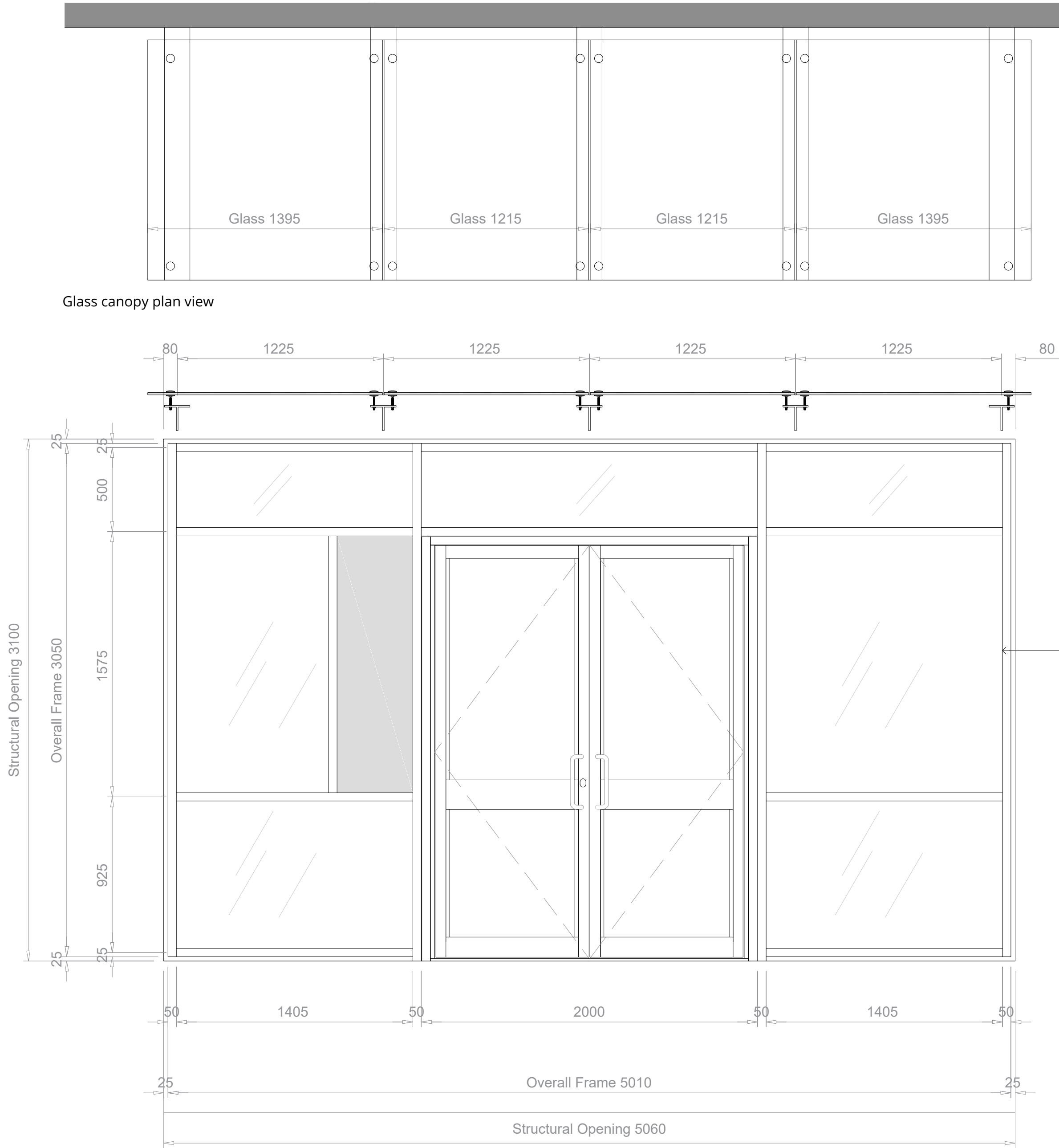
New double door and glass side panel elevation
