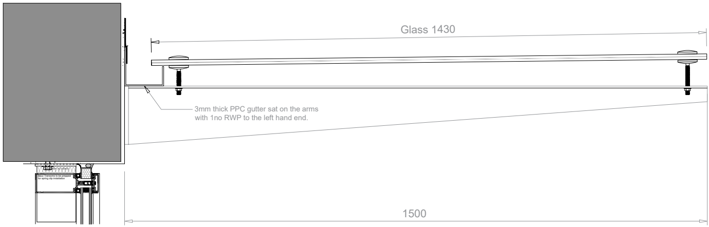
Section through proposed glass canopy
