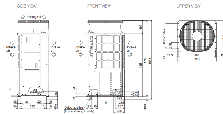
Outdoor VRF Equipment
