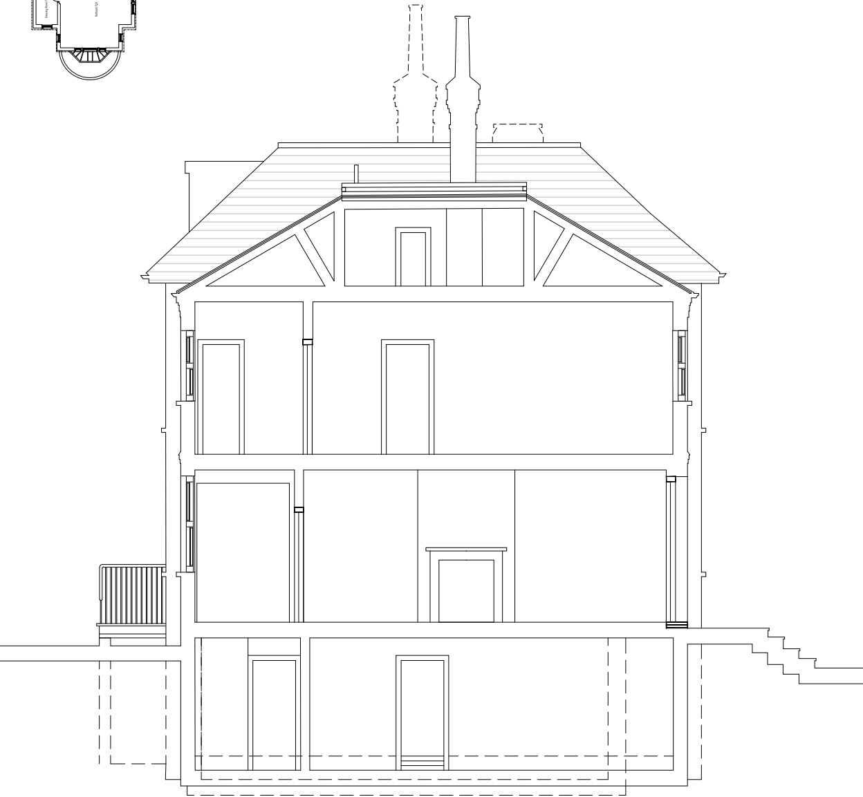
Section: Existing
