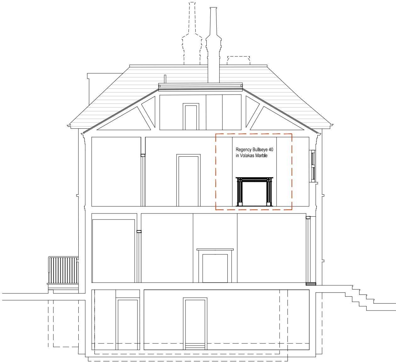
Section: Proposed
