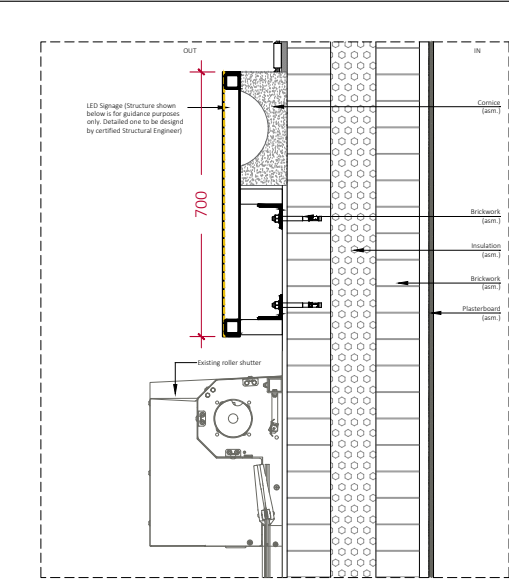
DETAIL 01 SIGNAGE LOCATION SCALE 1:20
