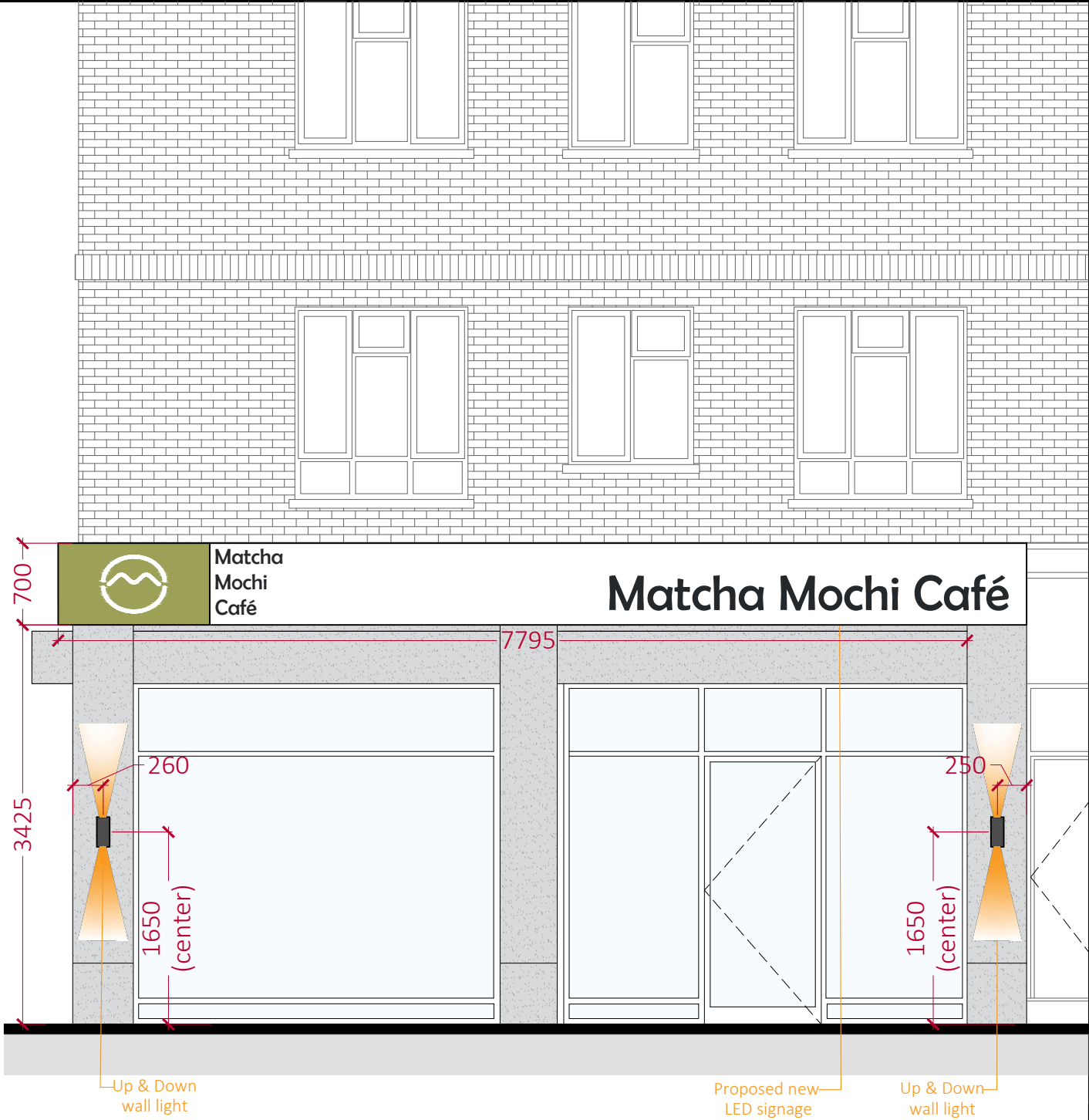
PROPOSED FACADE & SIGNAGE LOCATION ELEVATION SCALE 1:50
