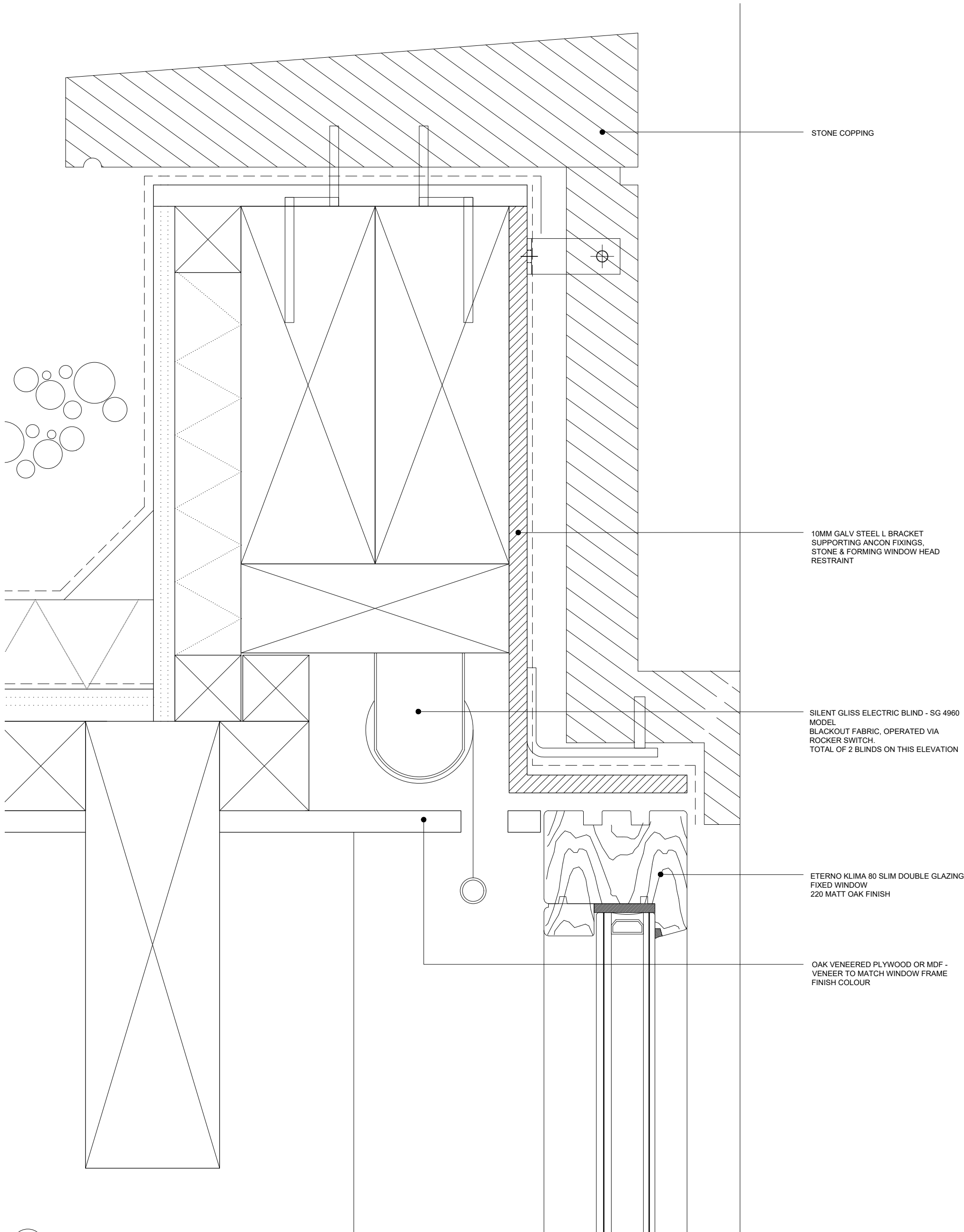
PROPOSED TOP LIGHT & PARAPET DETAIL 1:2 @A3
