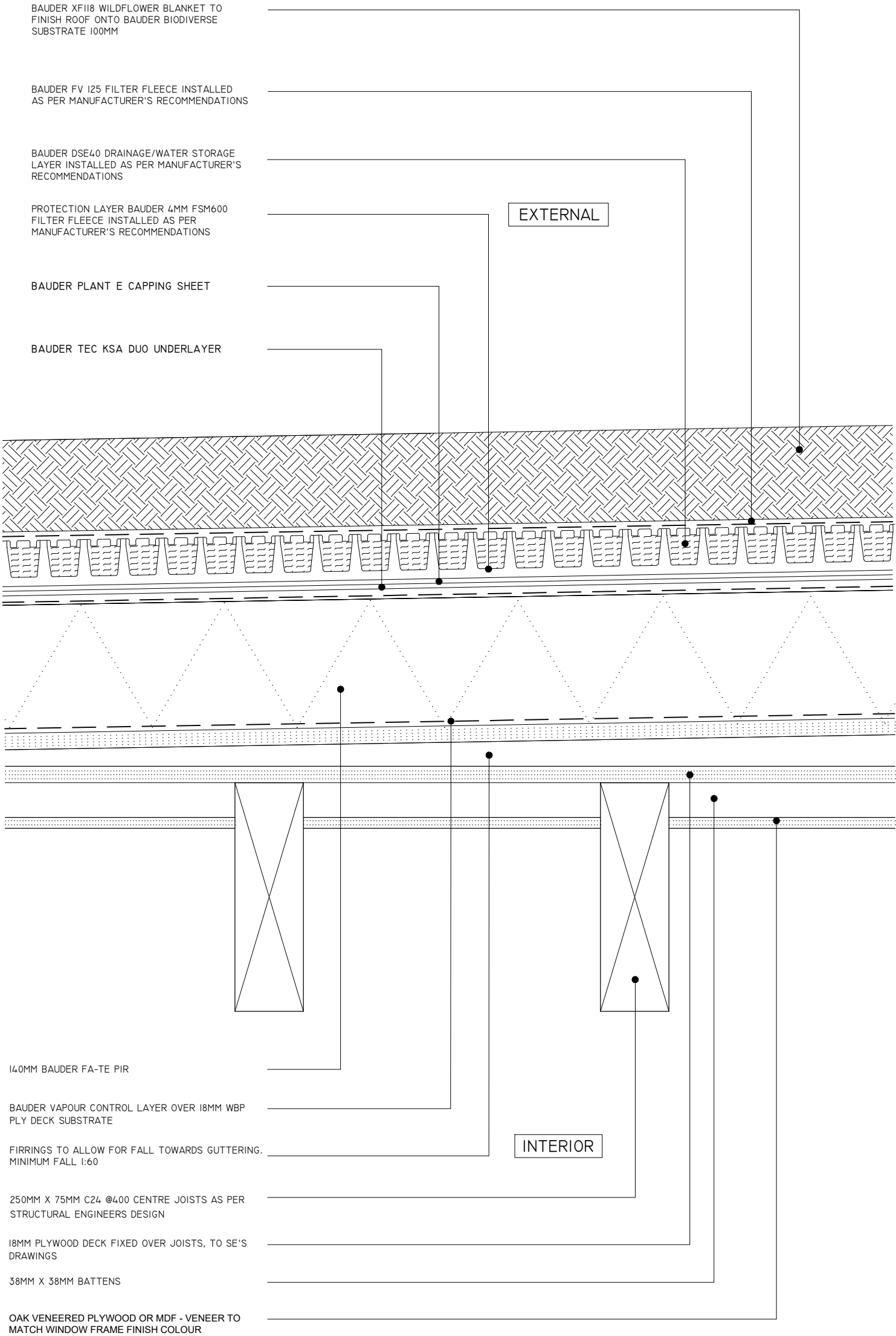
RTI EXTENSION GREEN ROOF BUILD UP
