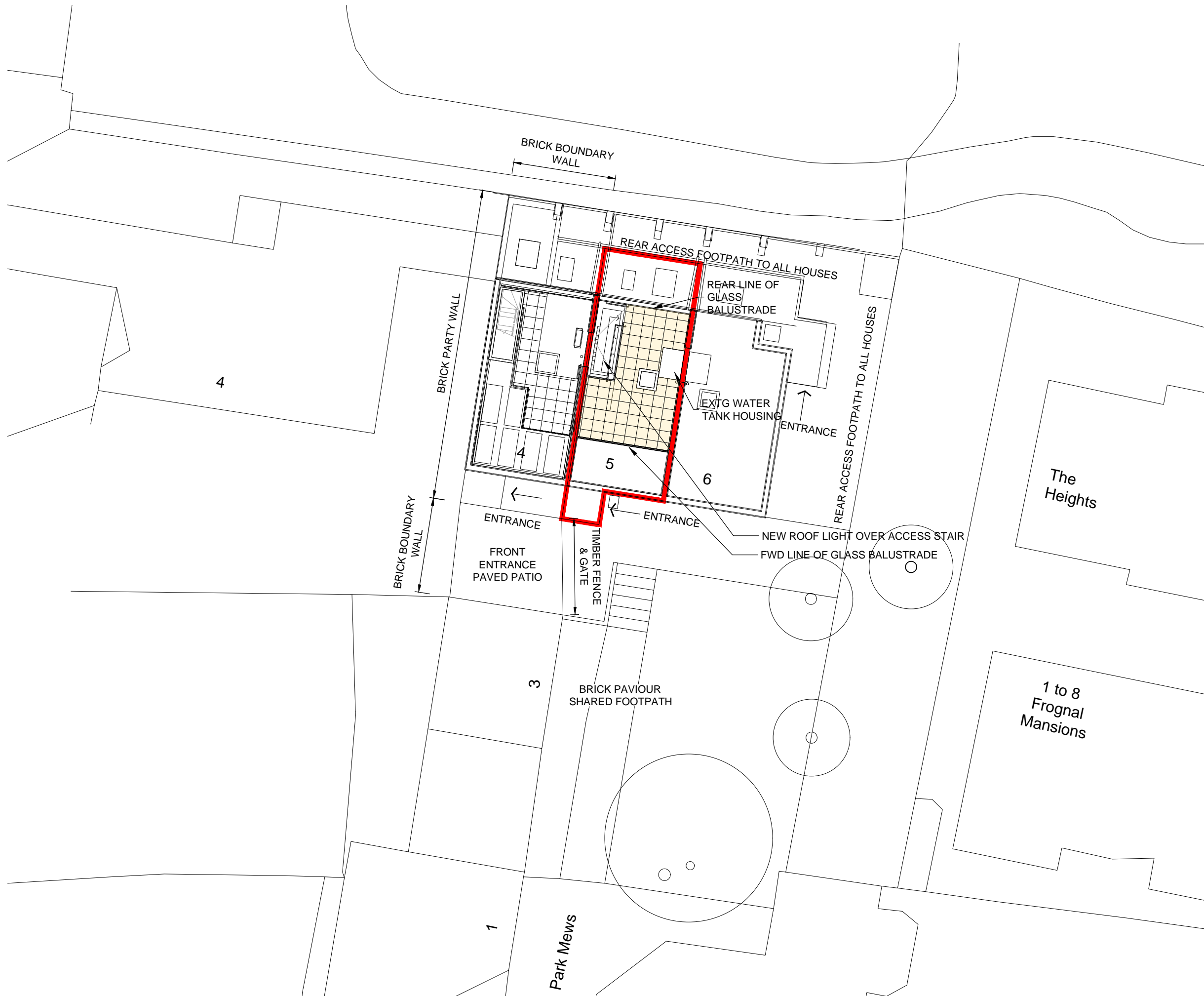
1 PROPOSED SITE PLAN
