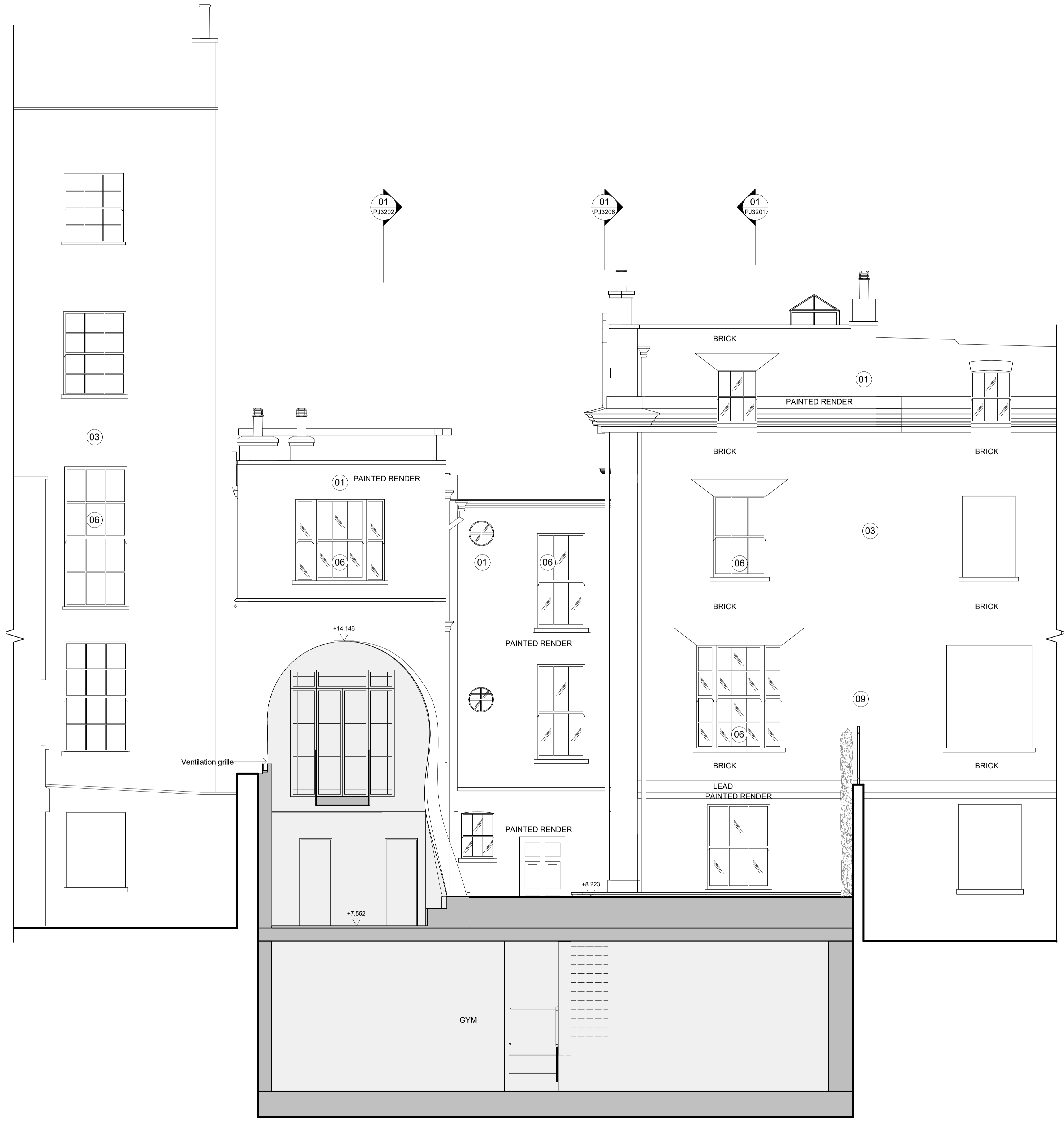
01 Proposed Section F Link 1 : 50
