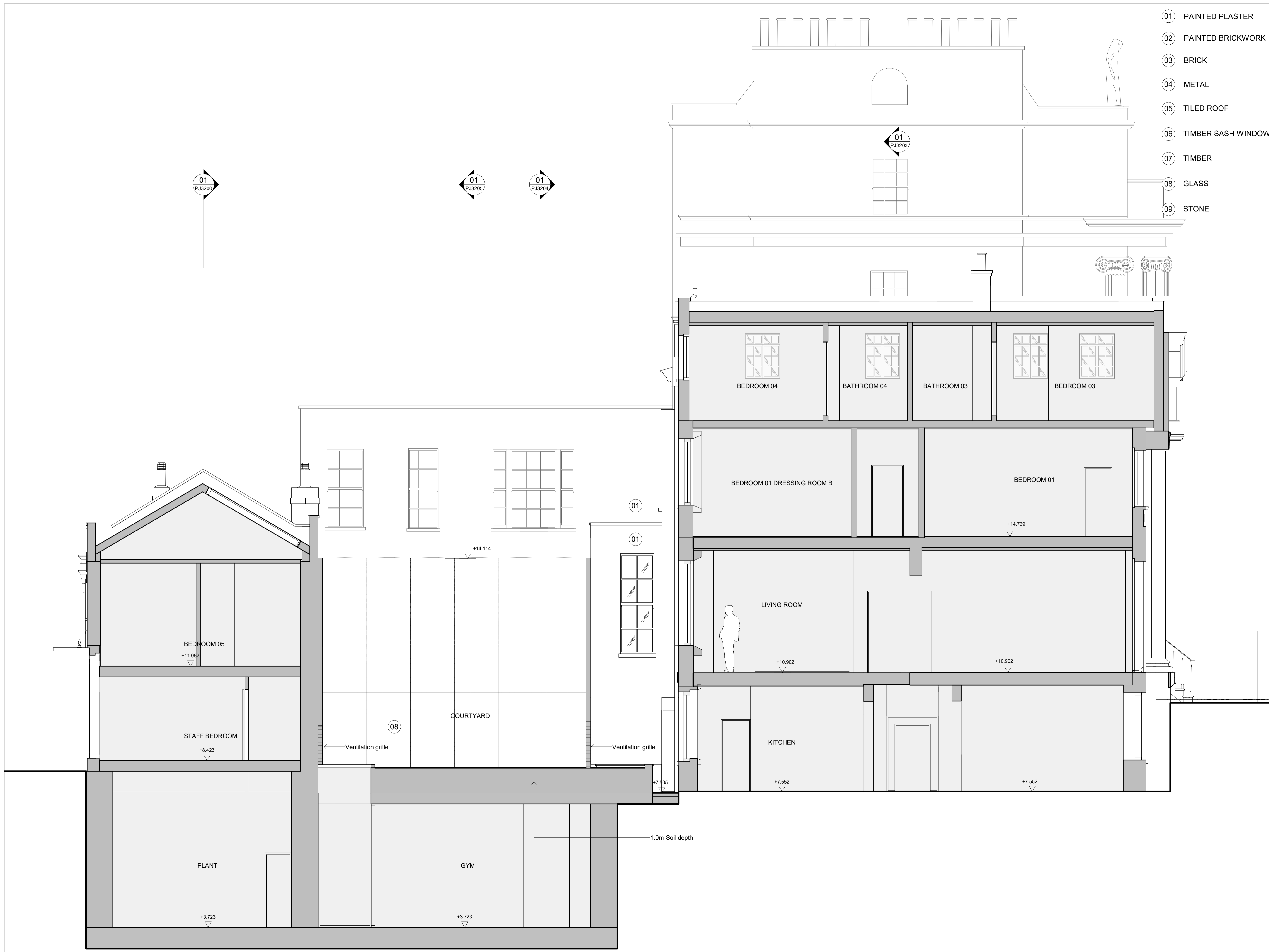
01 Proposed Section B Link 1 : 50
