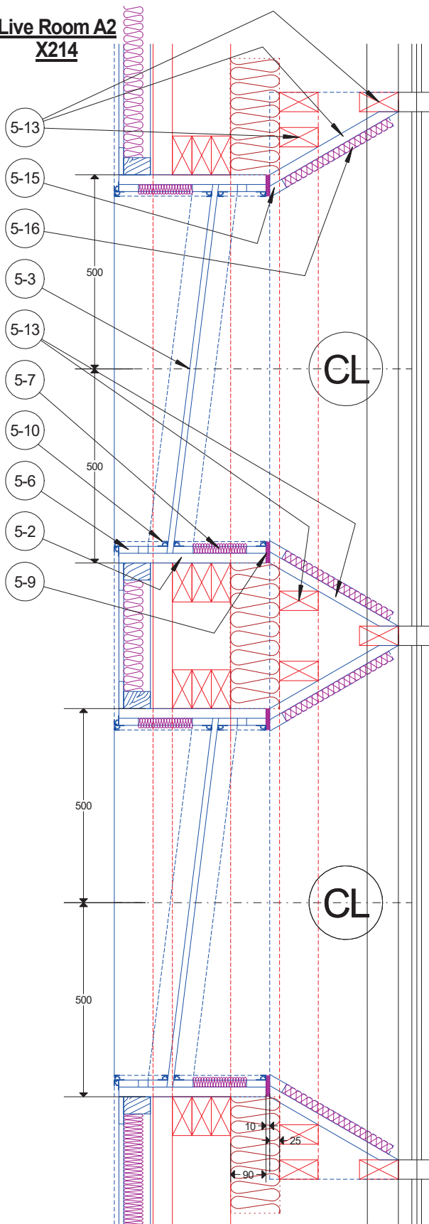
Plan Section
