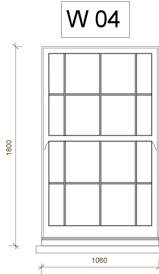
EXTERNAL ELEVATION
