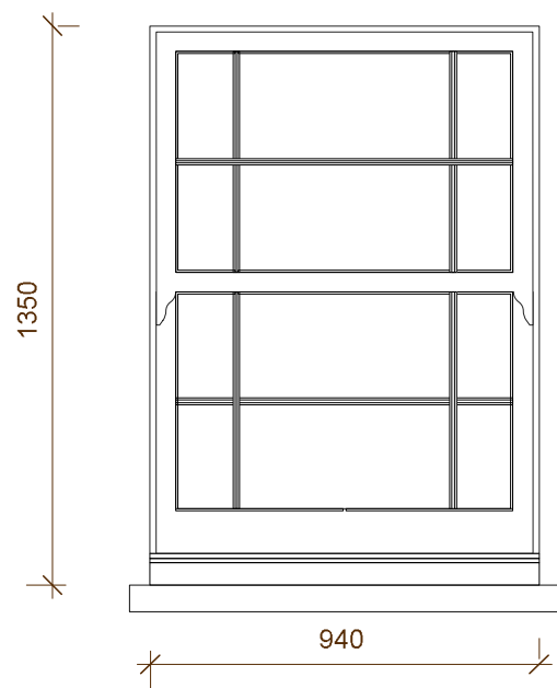
EXTERNAL ELEVATION
