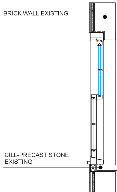
SECTION
