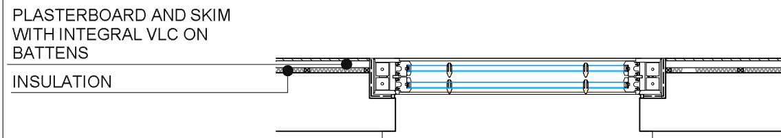
PLAN
