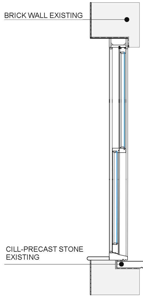
SECTION
