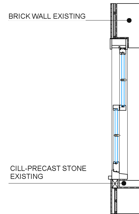
SECTION
