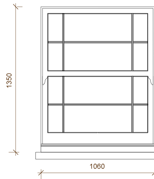
EXTERNAL ELEVATION
