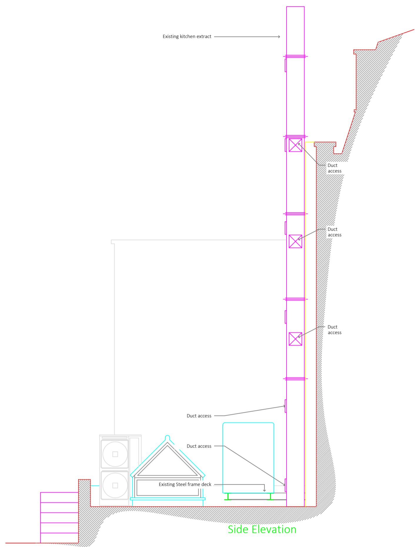
SIDE ELEVATION
