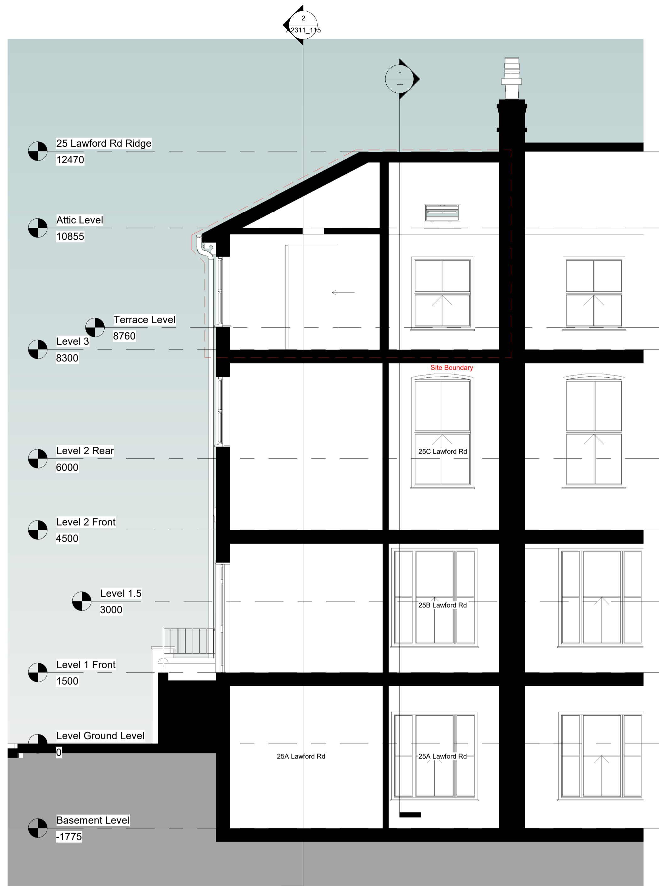
1 Proposed Section A-A 1 : 50
