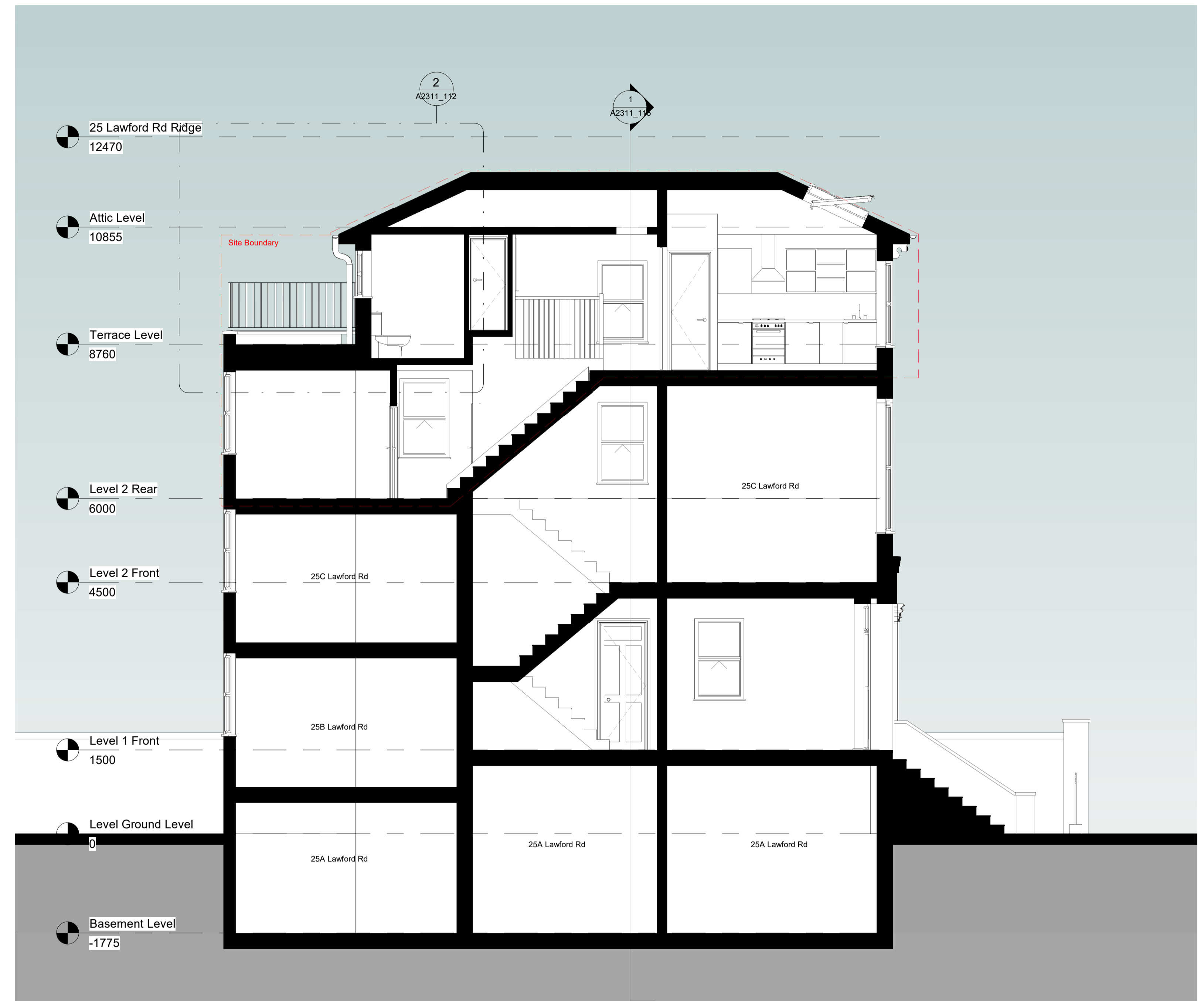
2 Proposed Section B-B 1 : 50
