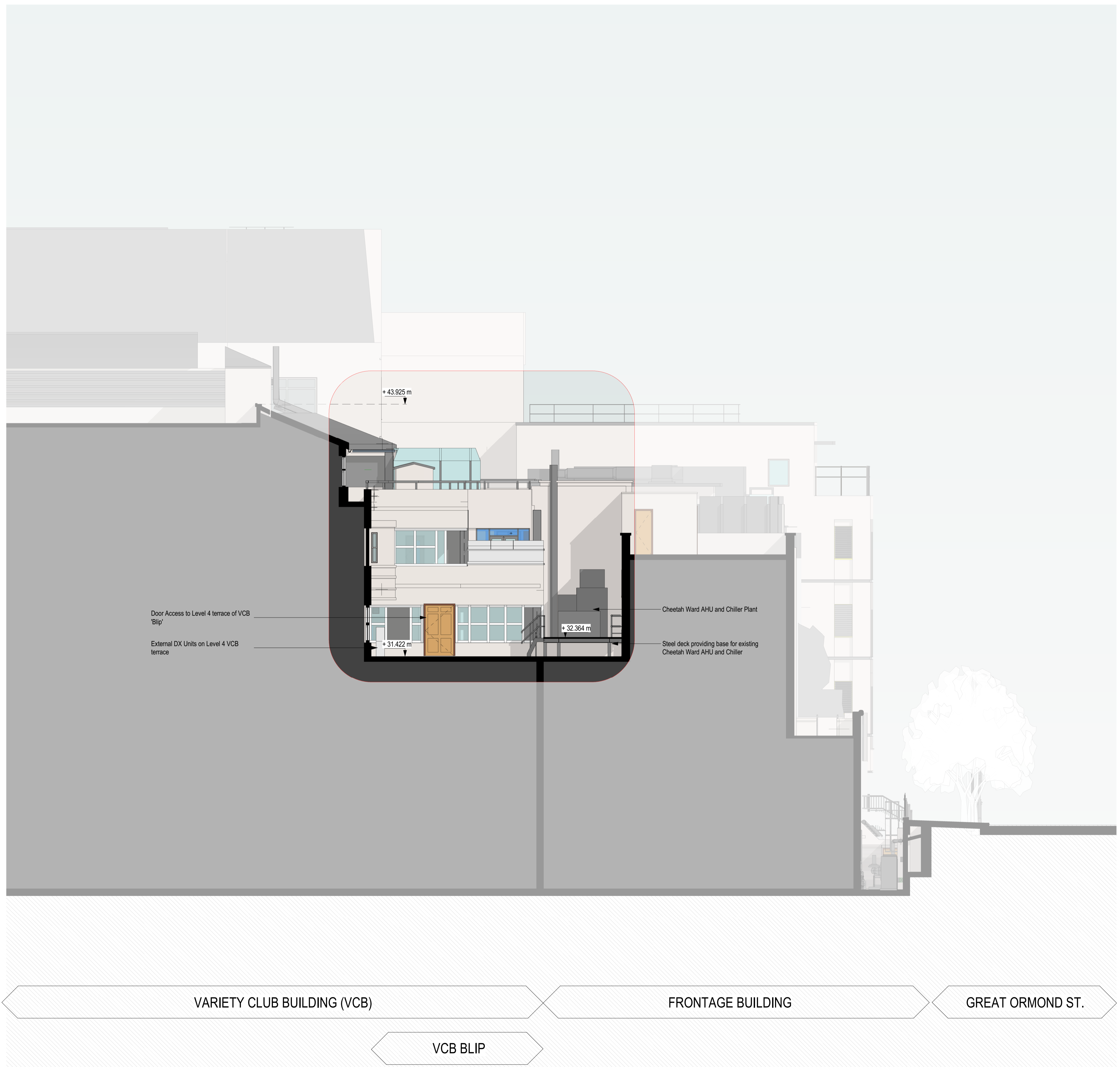
1 East Facing Blip Sectional Elevation - Existing 1 : 100
