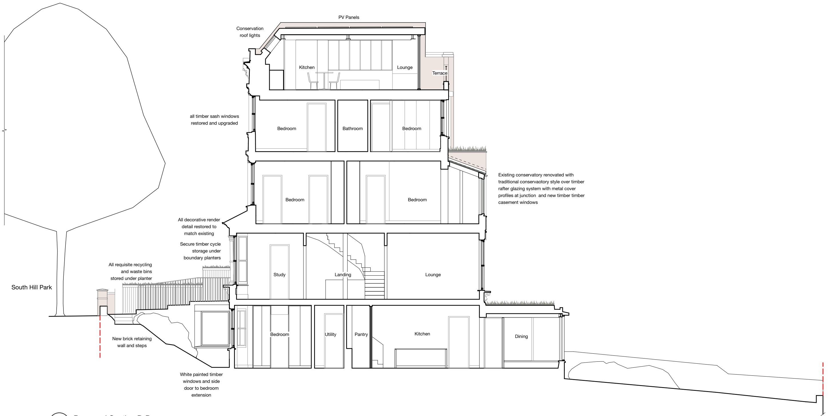
1 Proposed Section D-D Scale: 1:100
