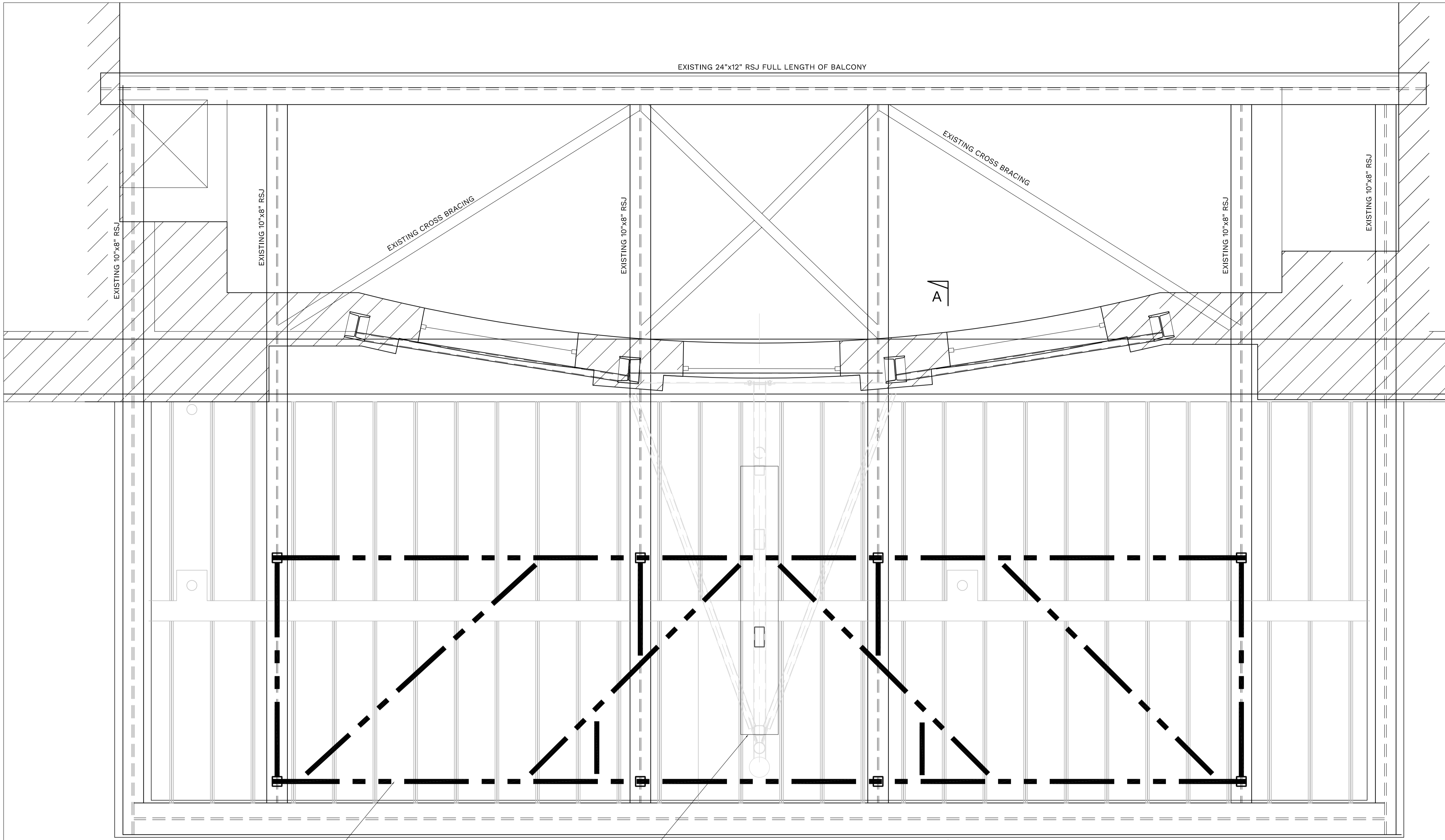
EXISTING CANOPY PLAN WITH STEELWORK OVER CANOPY (SCALE 1:20 AT A1)
