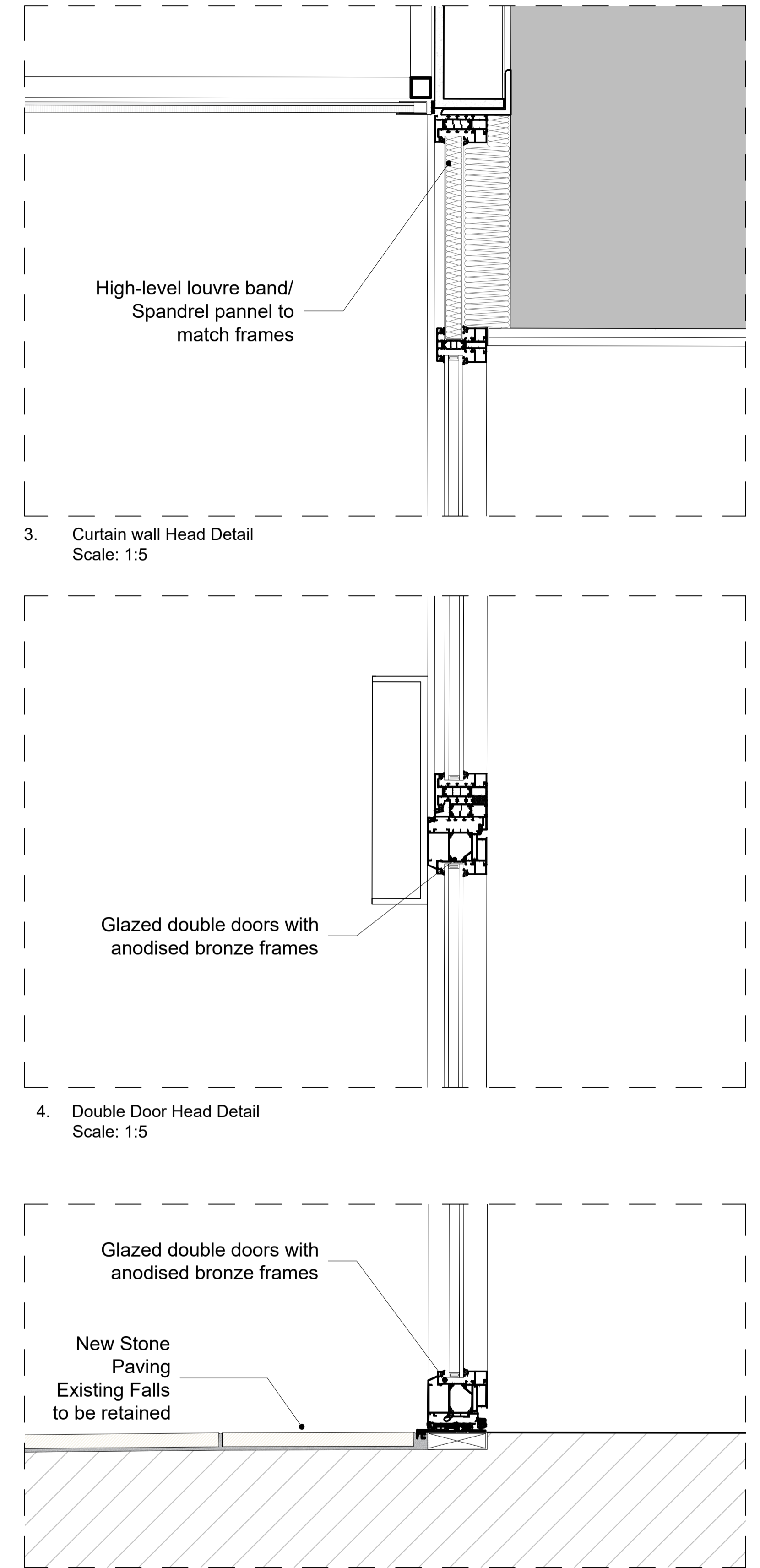
5. Double Door Sill and Paving Detail Scale: 1:5
