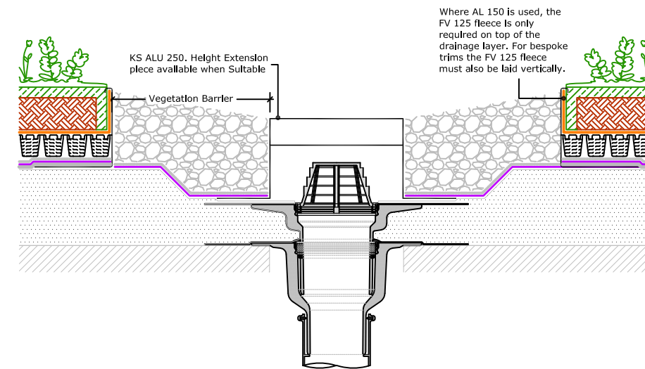
Bauder Outlet - Compact (Drg.No: D0901/03-00W_0-4Deg_006-ExtInt-S-DB_001)
