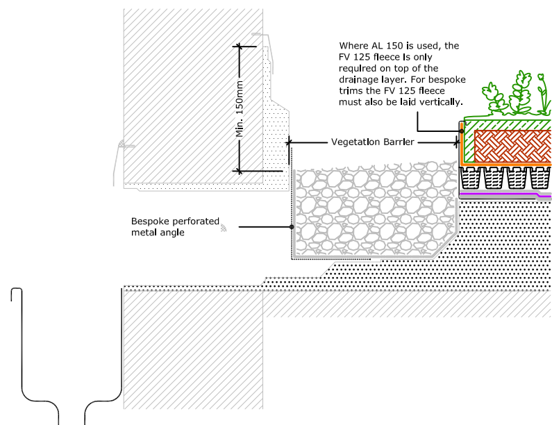
Upstand - Lead Chute (Drg.No: D0901/03-00W_0-4Deg_206-ExtInt-S-DB_002)
