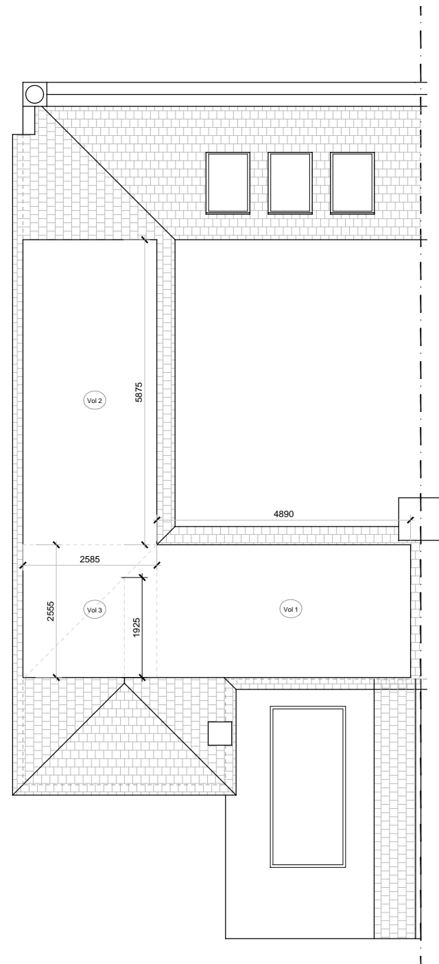
ROOF PLAN (proposed)
