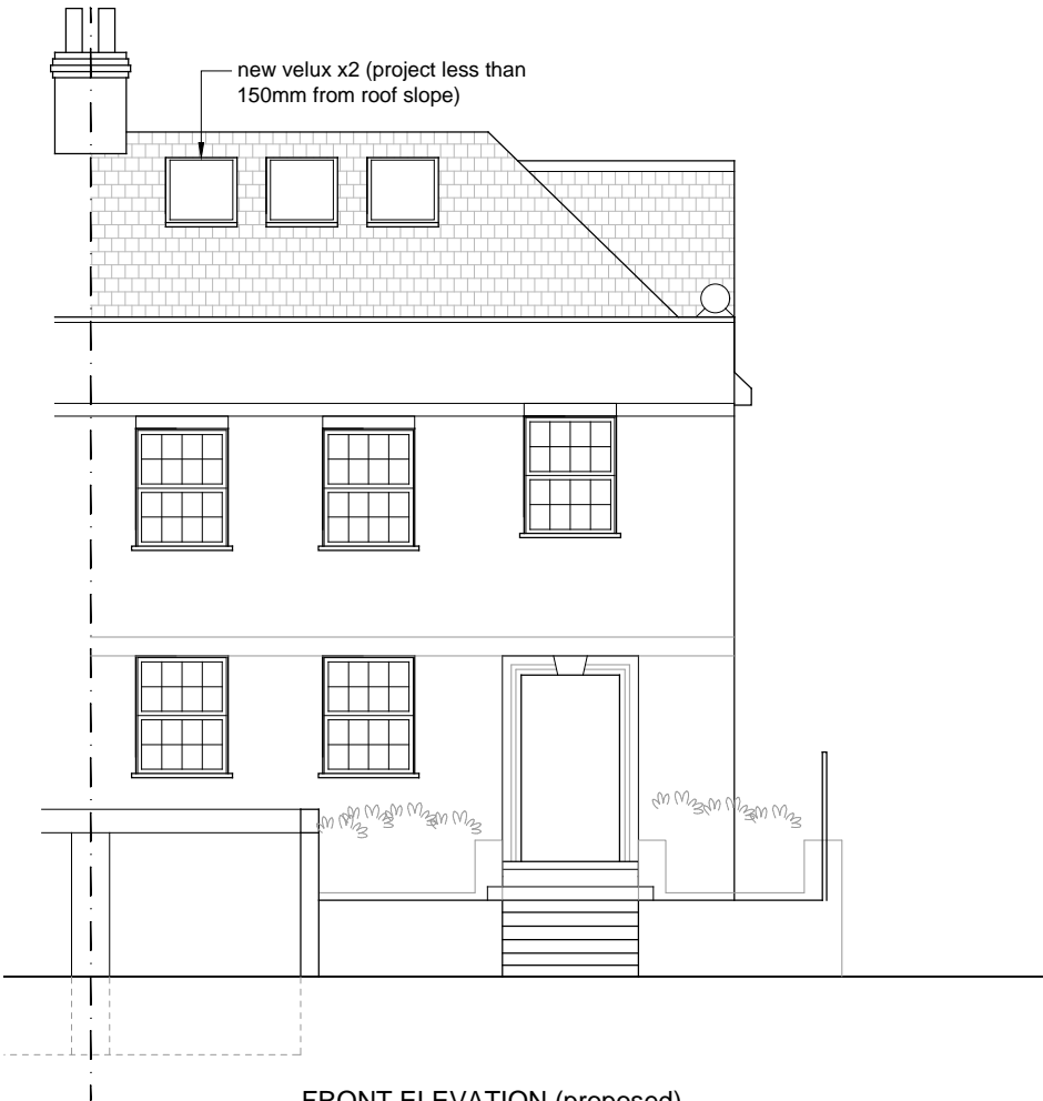
FRONT ELEVATION (proposed) boundary treatment in grey
