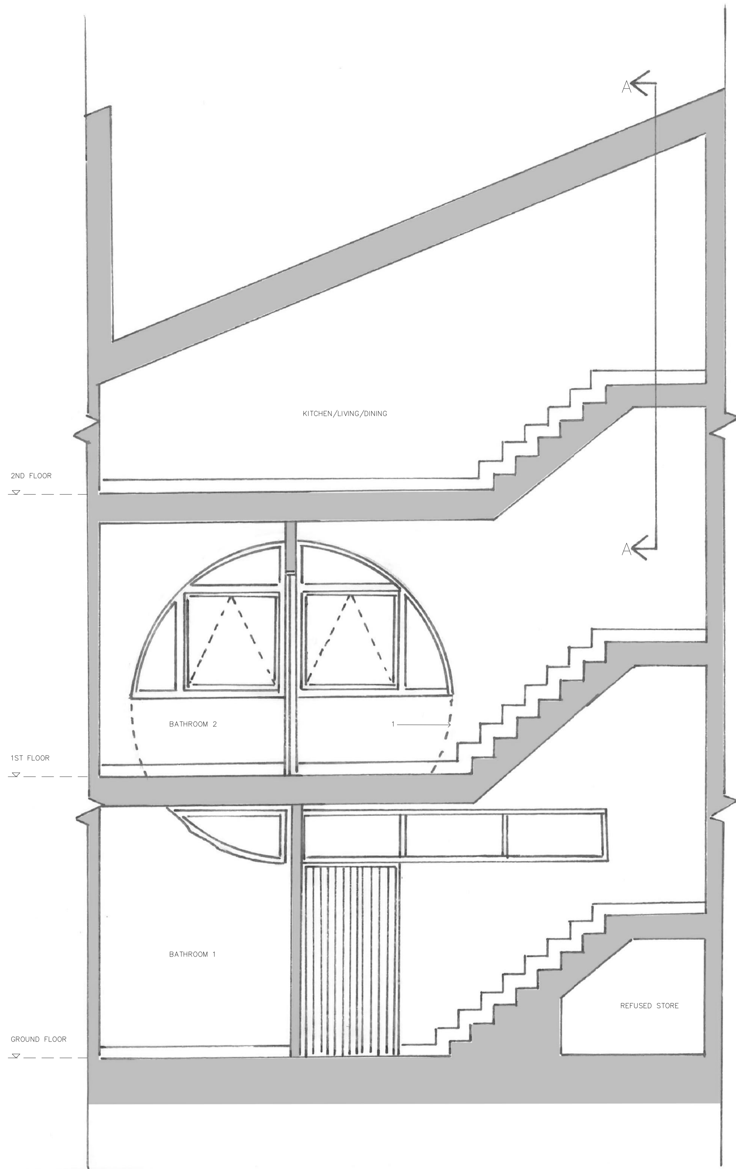
1:50 (@ A3) HOUSE 12, SECTION FACING NORTH
