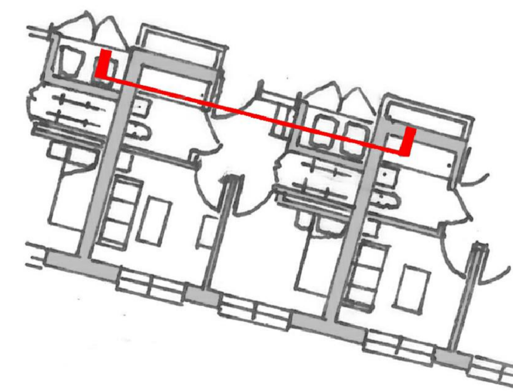
1:200 (@ A3) KEY PLAN
