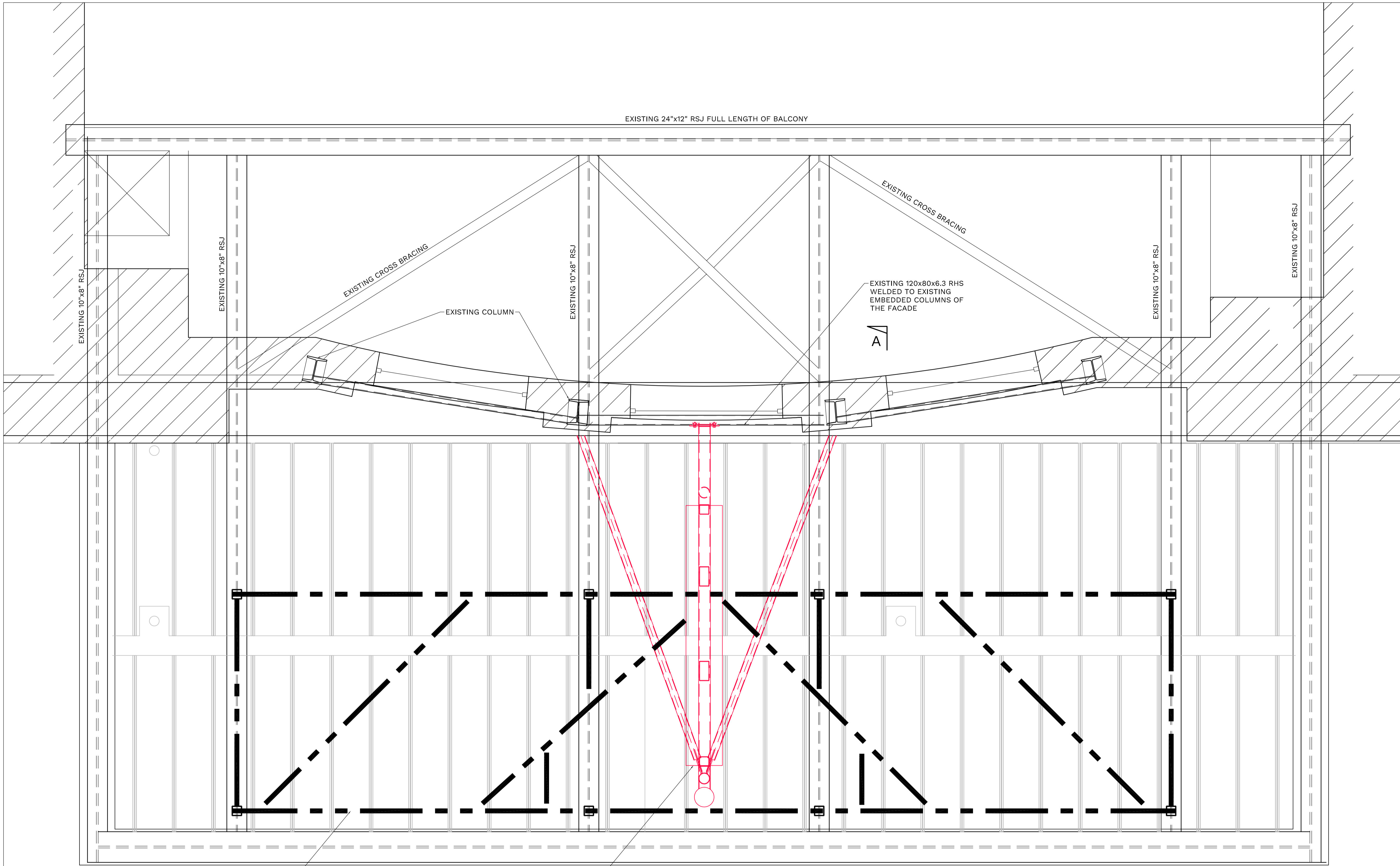
EXISTING CANOPY PLAN NOTING ITEMS TO BE REMOVED (SCALE 1:20 AT A1)
