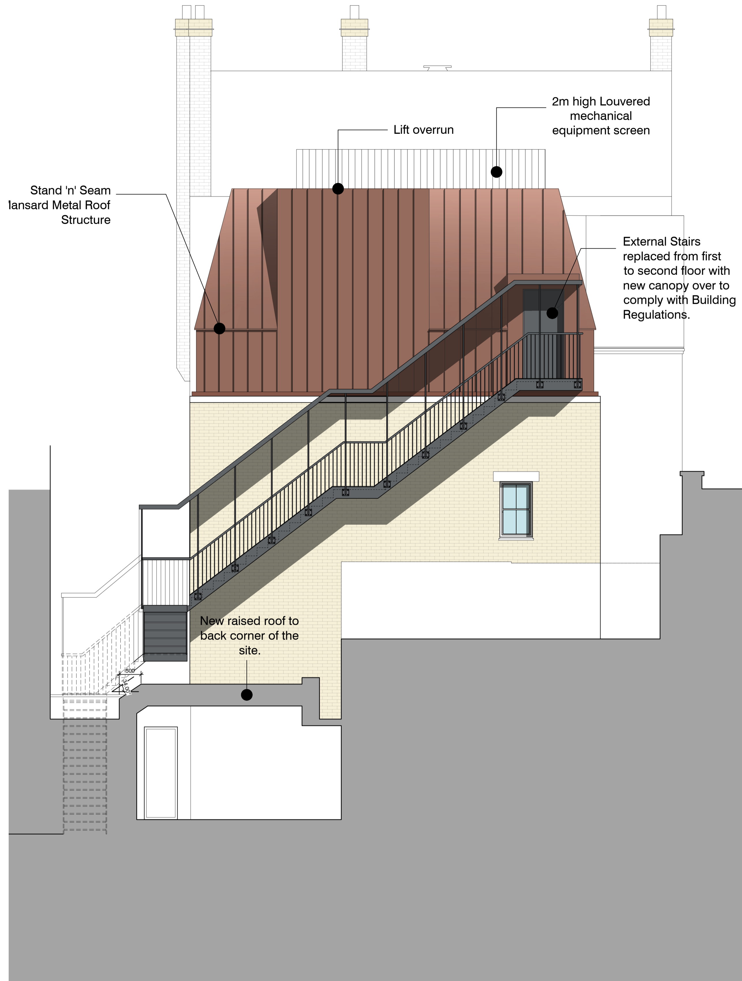
West Elevation
