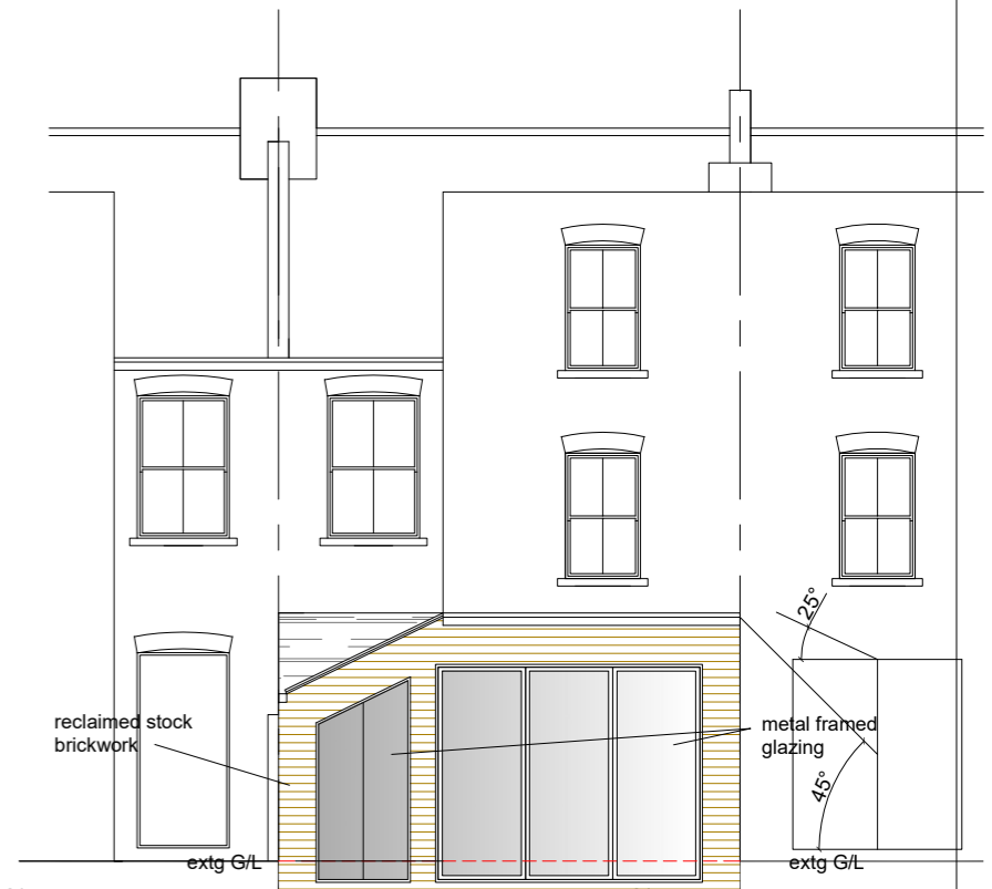
REAR ELEVATION
