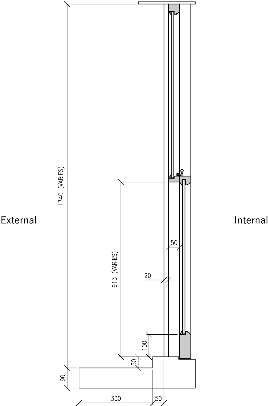
Typical Cross Section of Existing Sash Window
