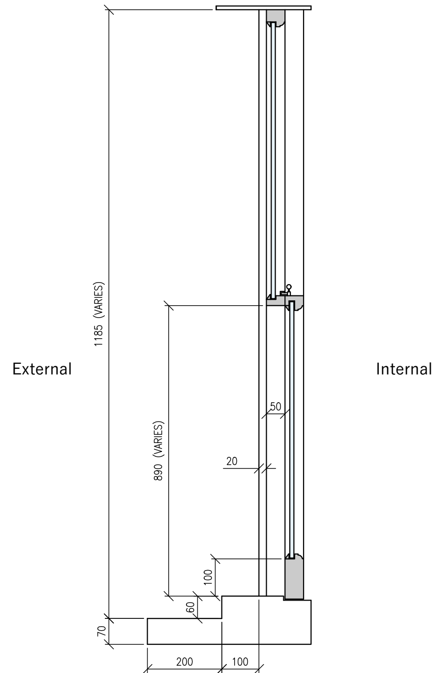
Typical Cross Section of Existing Sash Window
