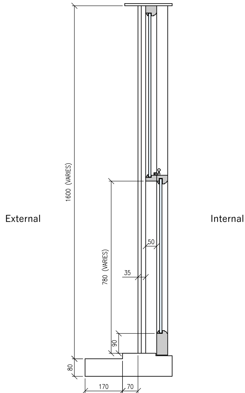
Typical Cross Section of Existing Sash Window
