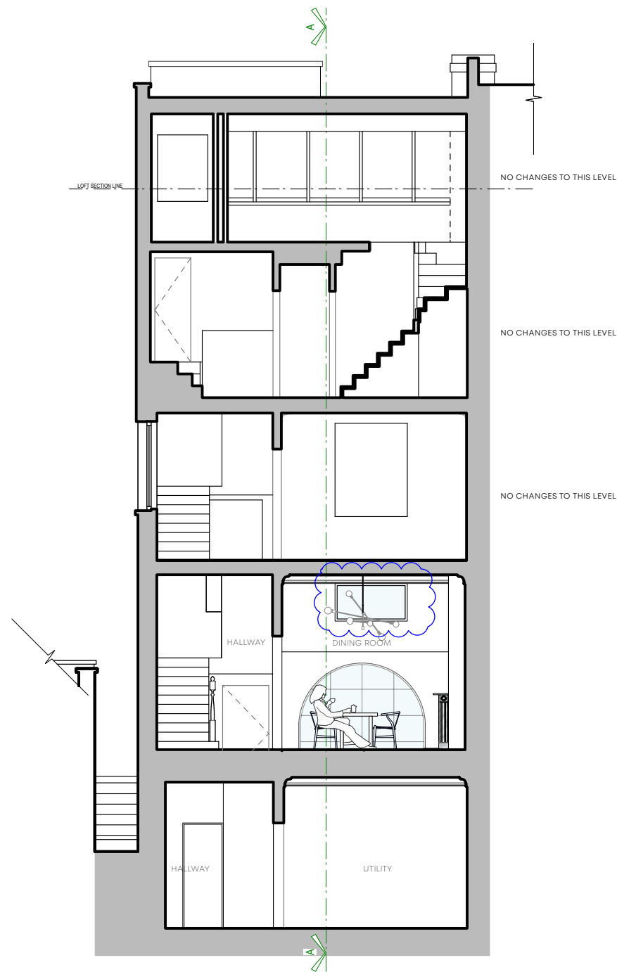
SECTION B-B
