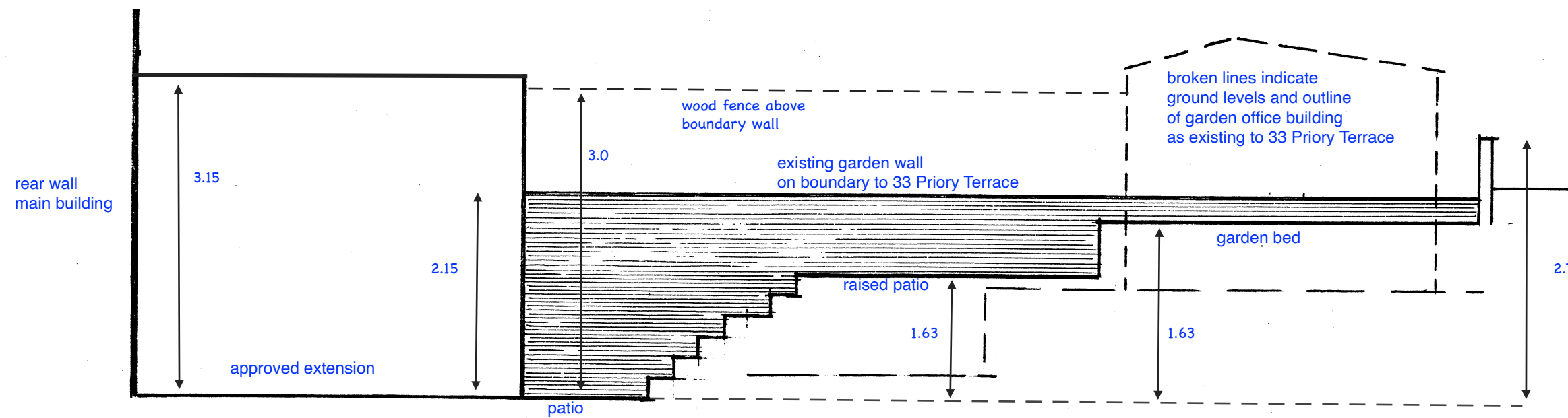
SITE SECTION THROUGH REAR GARDEN AS EXISTING
