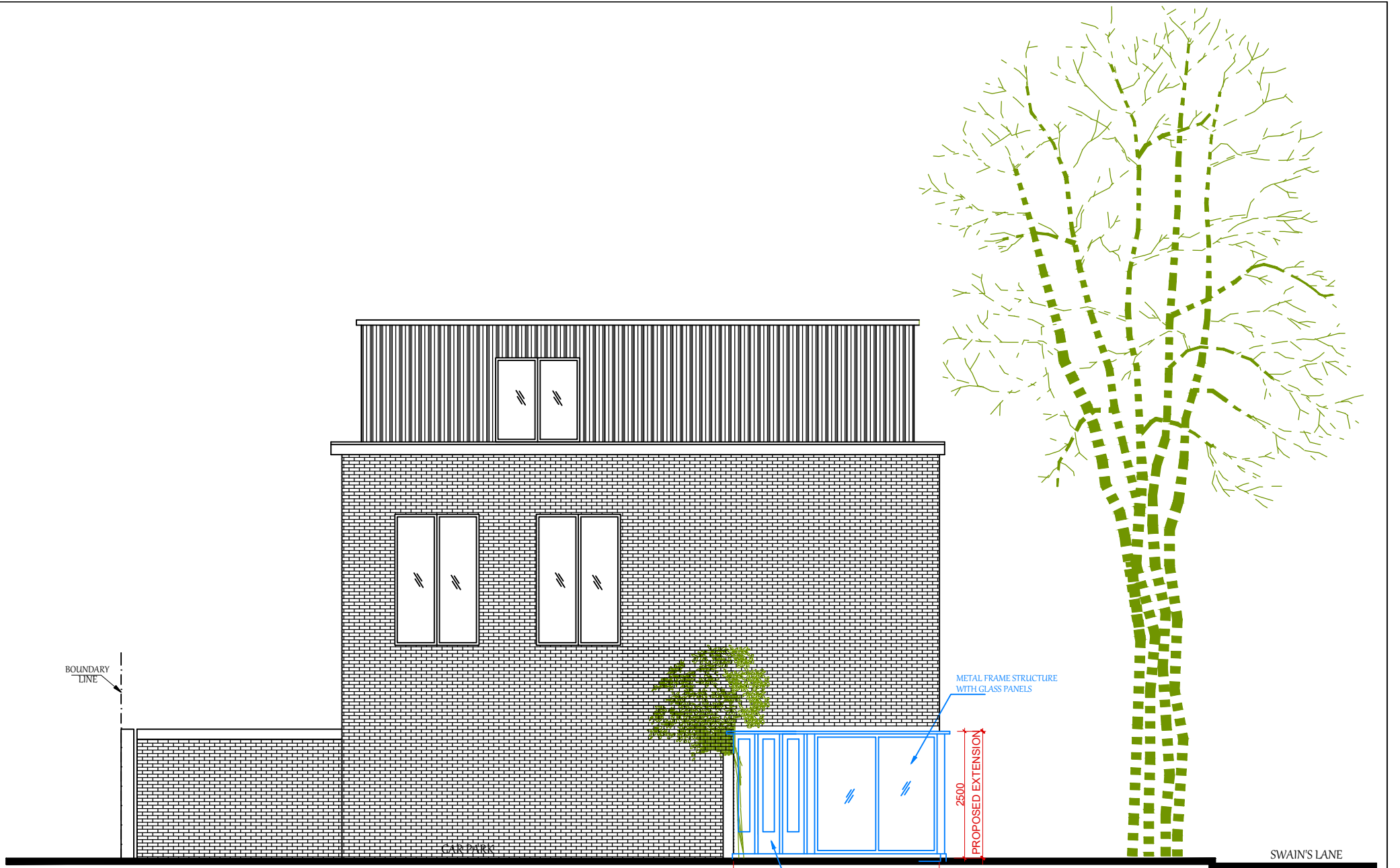
PROPOSED SIDE ELEVATION SCALE: 1/100 @A3
