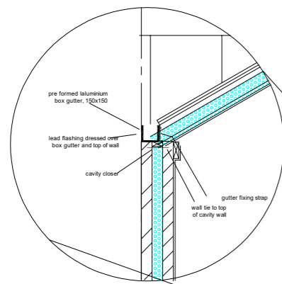
SECTION D GUTTER DETAIL
