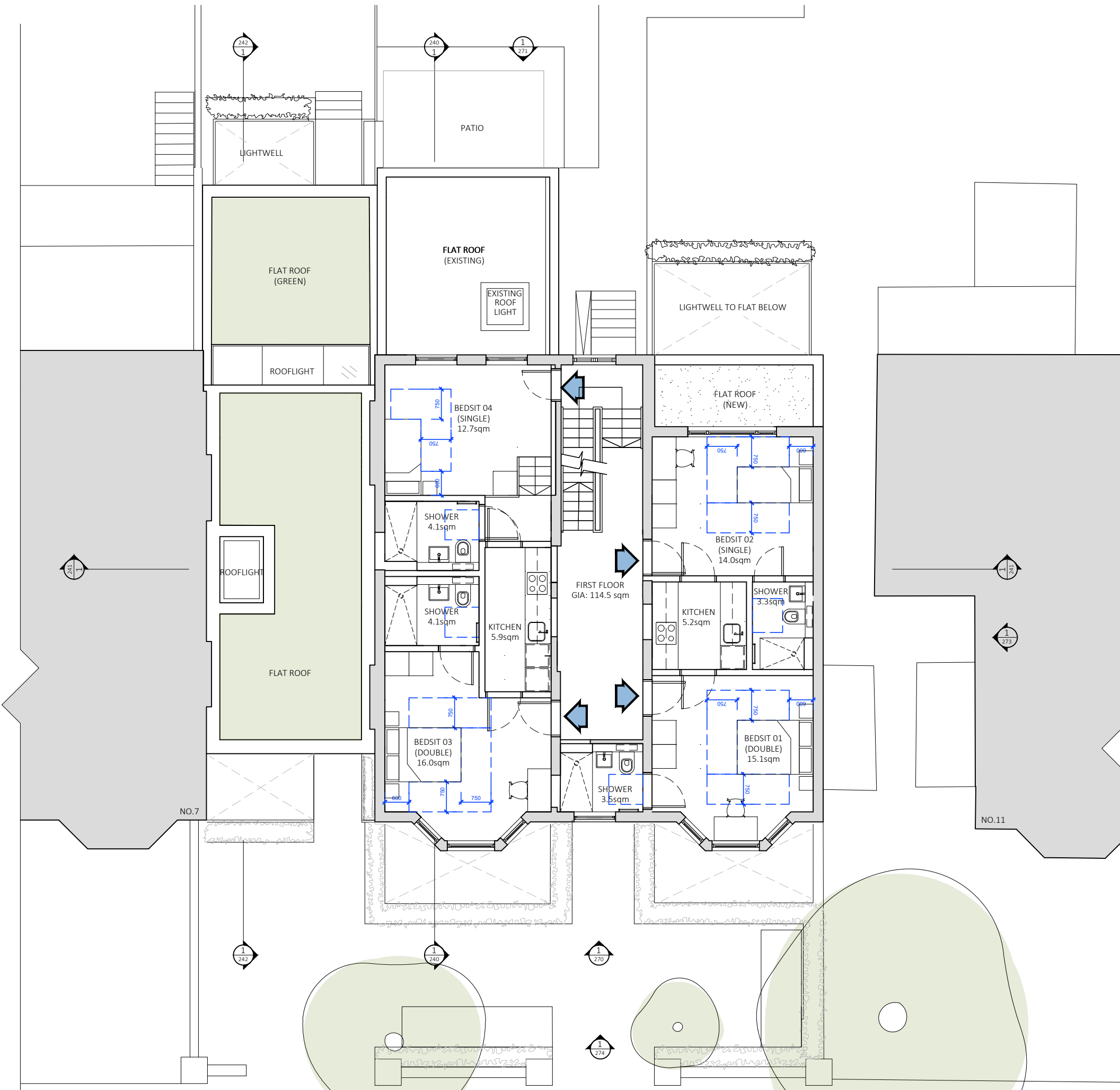
1 PROPOSED FIRST FLOOR PLAN 1:100 @ A3
