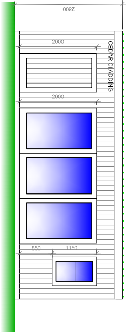
FRONT ELEVATION
