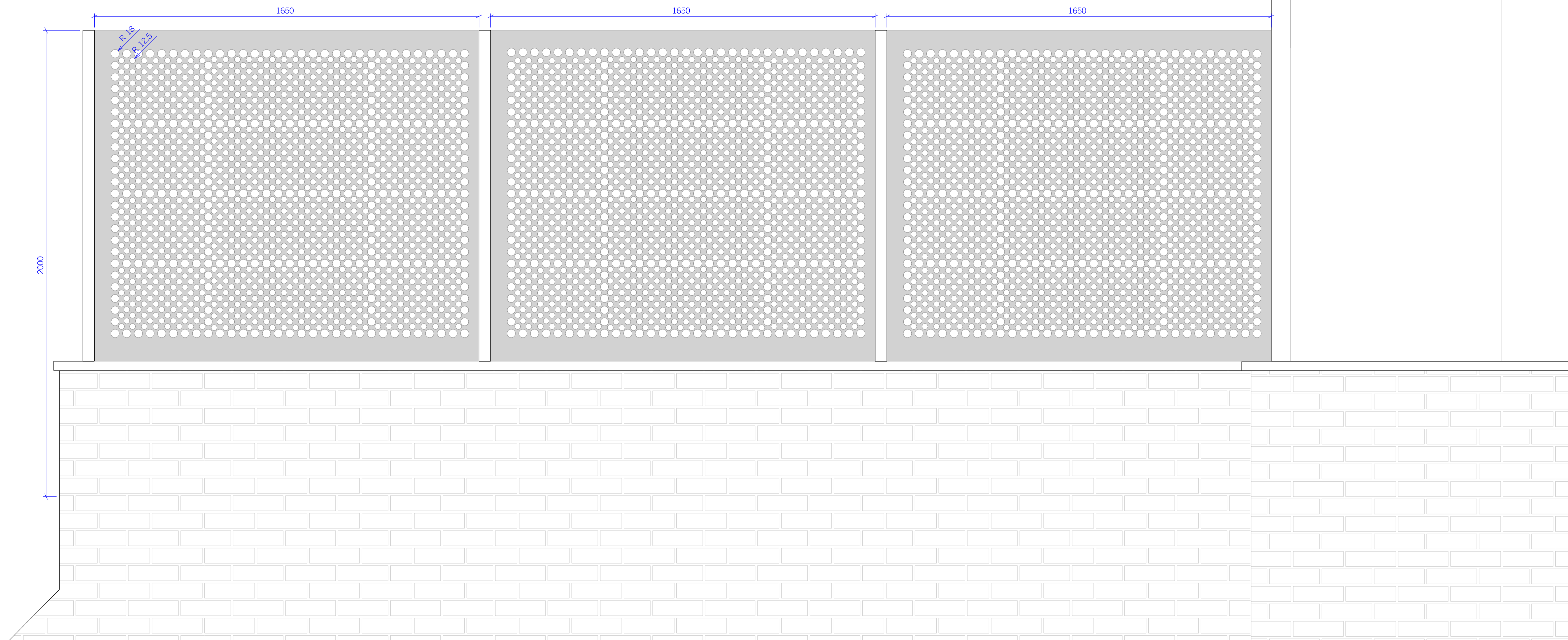
03: DETAILED PRIVACY SCREEN ELEVATION SCALE 1:10
