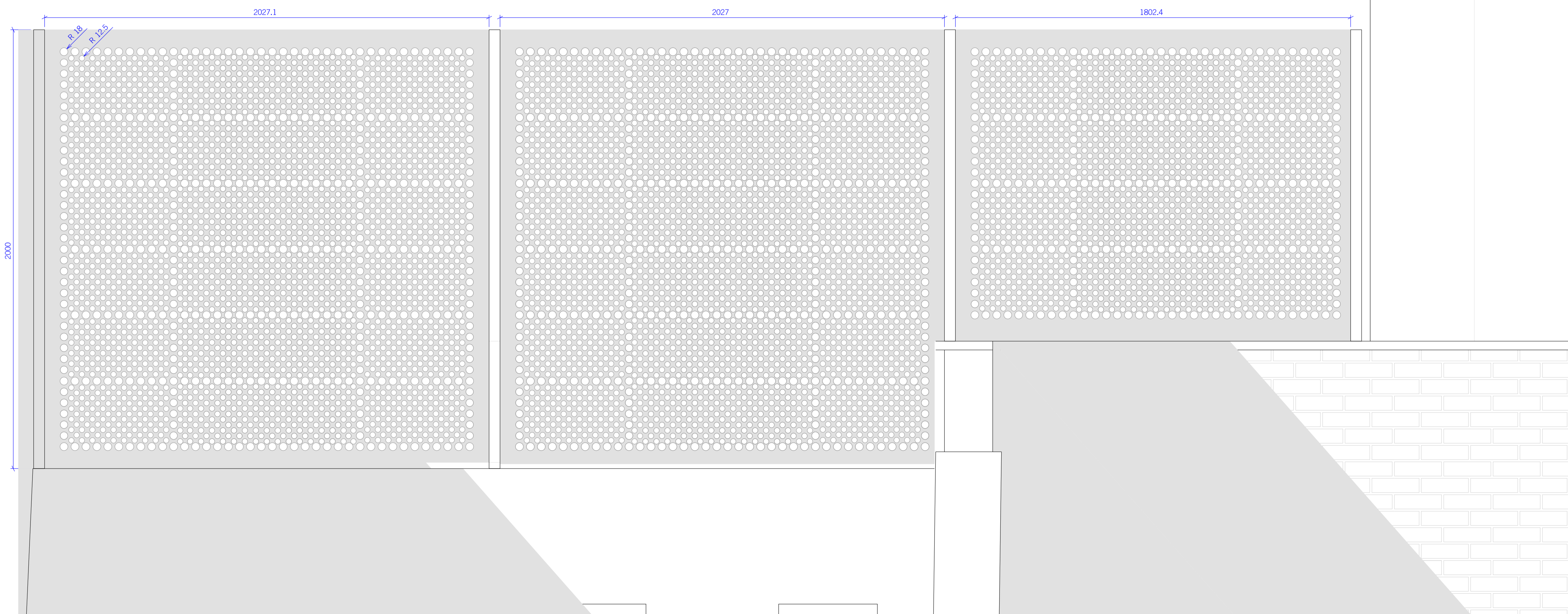
03: DETAILED PRIVACY SCREEN ELEVATION SCALE 1:10
